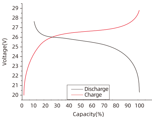
25.6V 100Ah Charge-Discharge Curve 0.5C, 25°C
