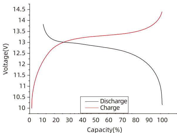
12.8V 150Ah Charge-Discharge Curve 0.5C, 25°C
