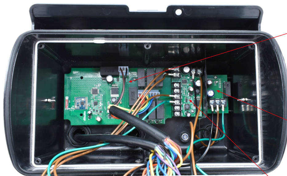
Wireless receiving module (optional)
