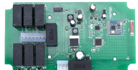
Wireless receiving module (optional)
