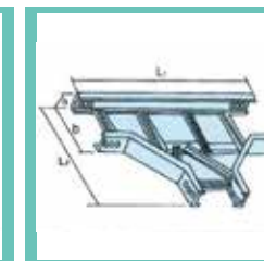
LADDER TYPE HORIZONTAL TEE
