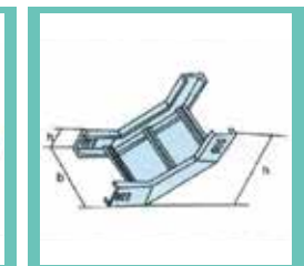
LADDER TYPE VERTICAL CON- CAVE BEND
