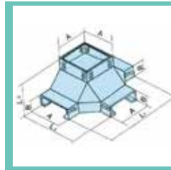
UPPER VERTICAL FOUR-WAY XQJ-C-D2
