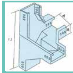
TOP LEFT VERTI- CAL FOUR-WAY XQJ-C-D7
