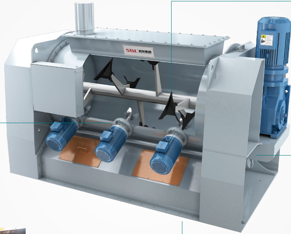
密封可靠的大开门出料口 Bomb door for discharge system with reliable seal 快速出料且无余料 Make fast discharge and no residues
