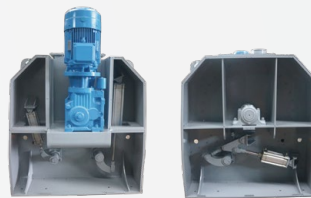
气动出料连杆 Auxiliary rod for pneumatic discharge system 停电后出料门不会打开 Ensure no open for bomb door if power failure
