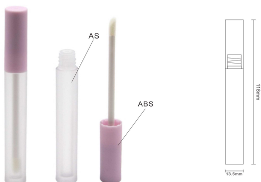
LG0487 Size:D13.5*H118mm Capacity:2ml Material :ABS+AS
