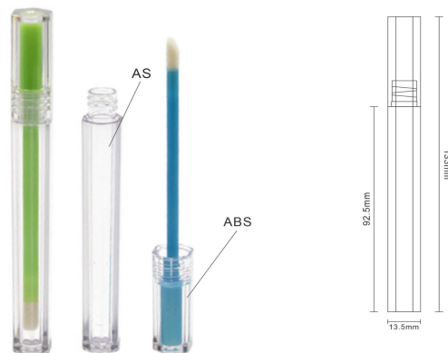
LG0488 Size:D13.5*H133mm Capacity:2.5ml Material :ABS+AS
