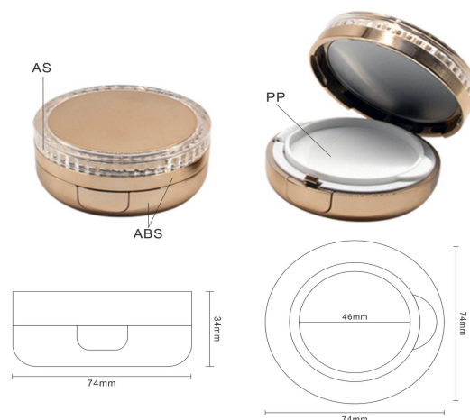
GS0555 Size:W74*H34mm Capacity:15g Material :AS+PP+ABS
