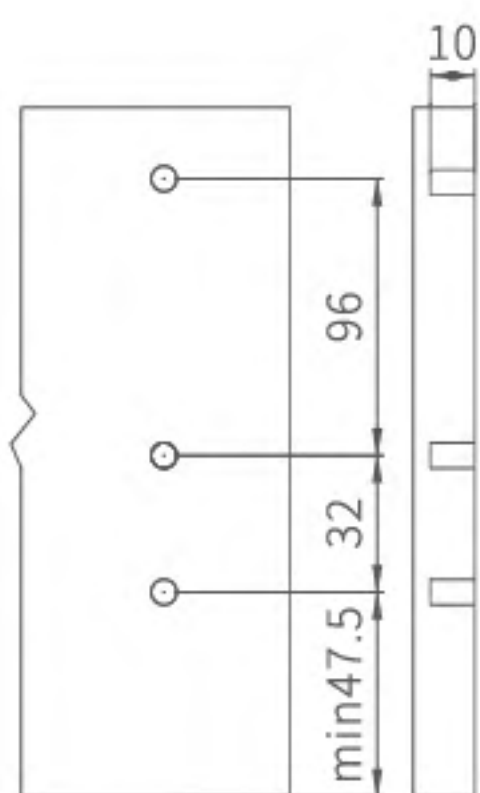
Panel hole size
