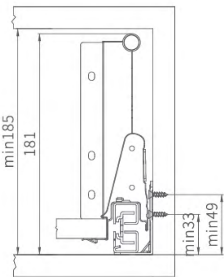
Space requirements of the inner cabinet installation
