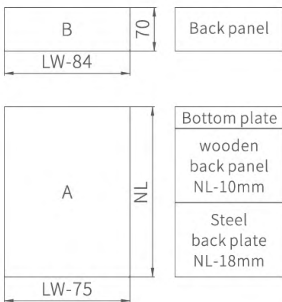
16mm(thickness)MDFcutting size
