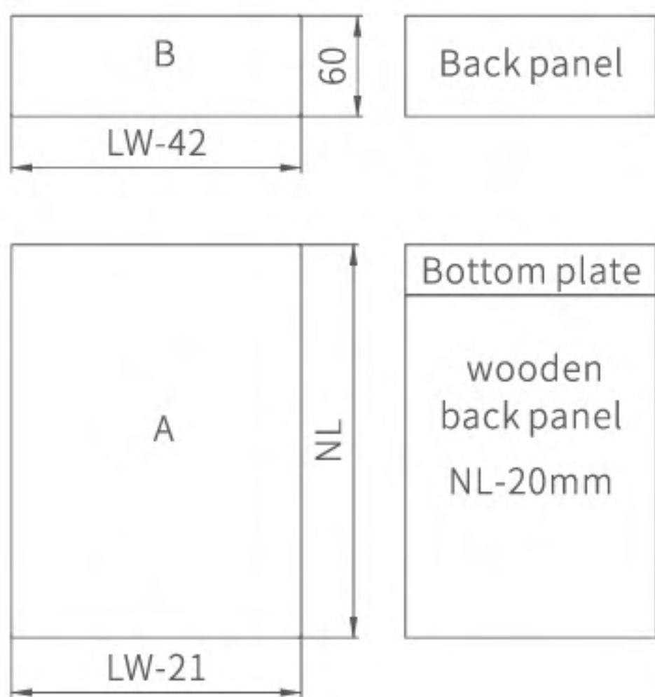
Slide mounting size
