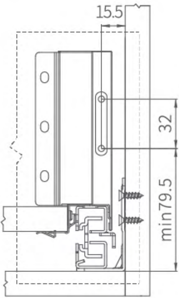
Front Connector panel mounting size
