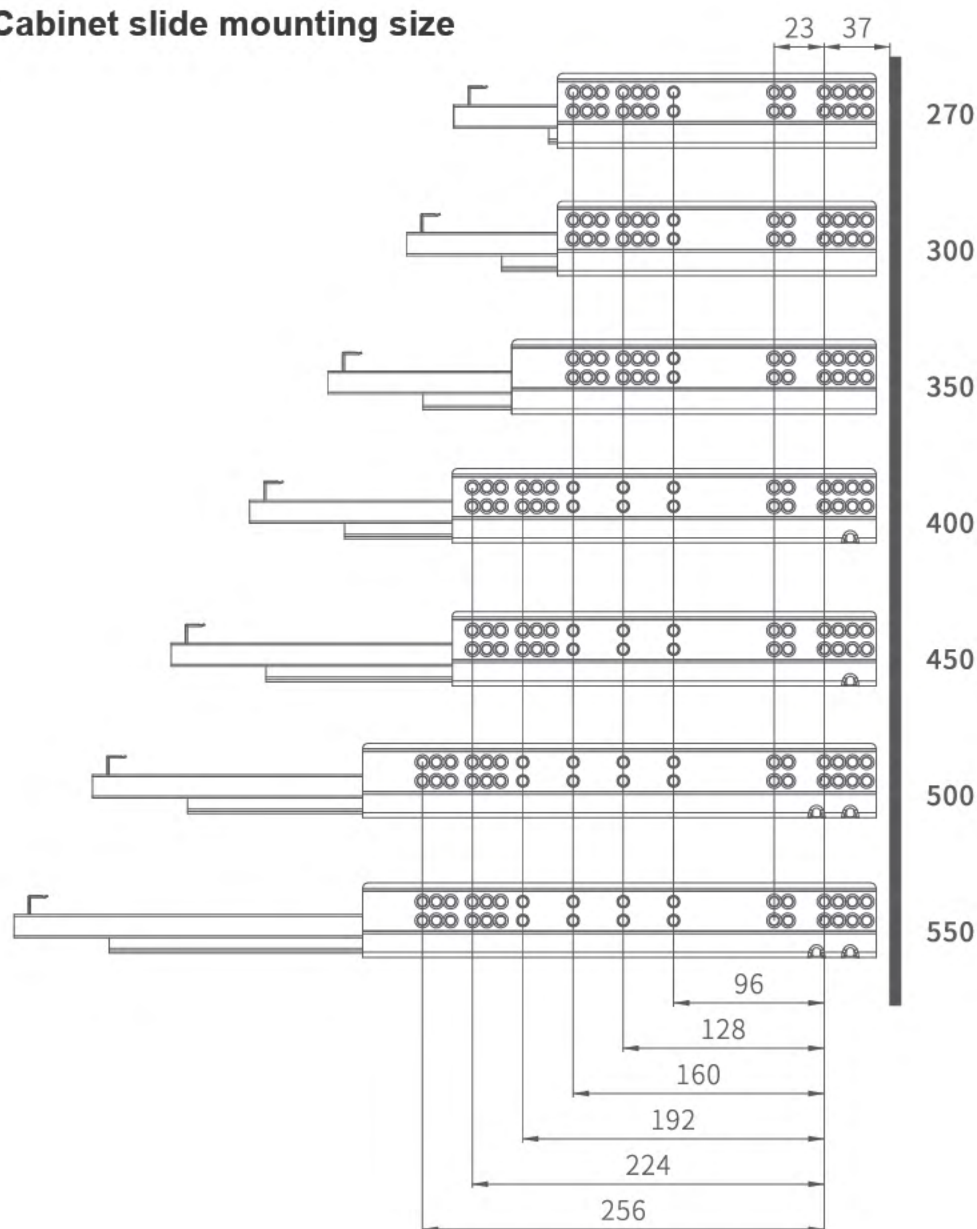
Cabinet slide mounting size
