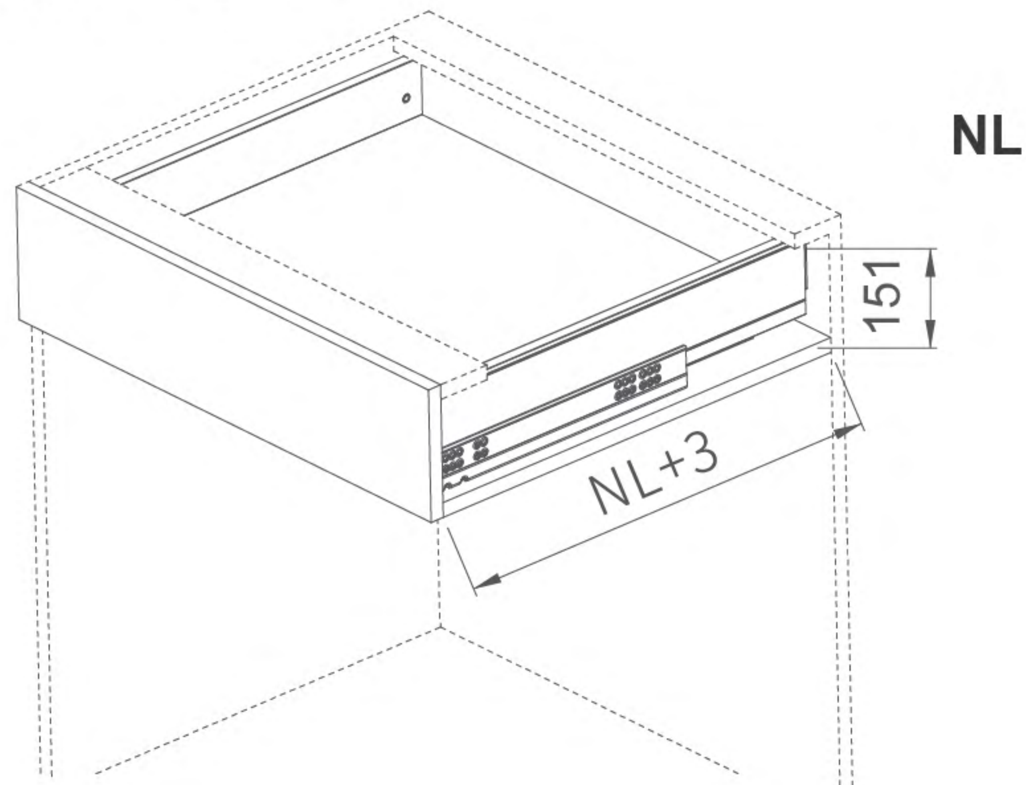
Space required
