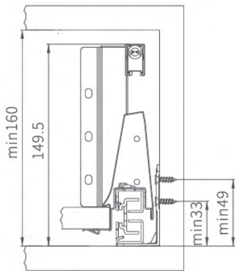
Space requirements of the inner cabinet installation
