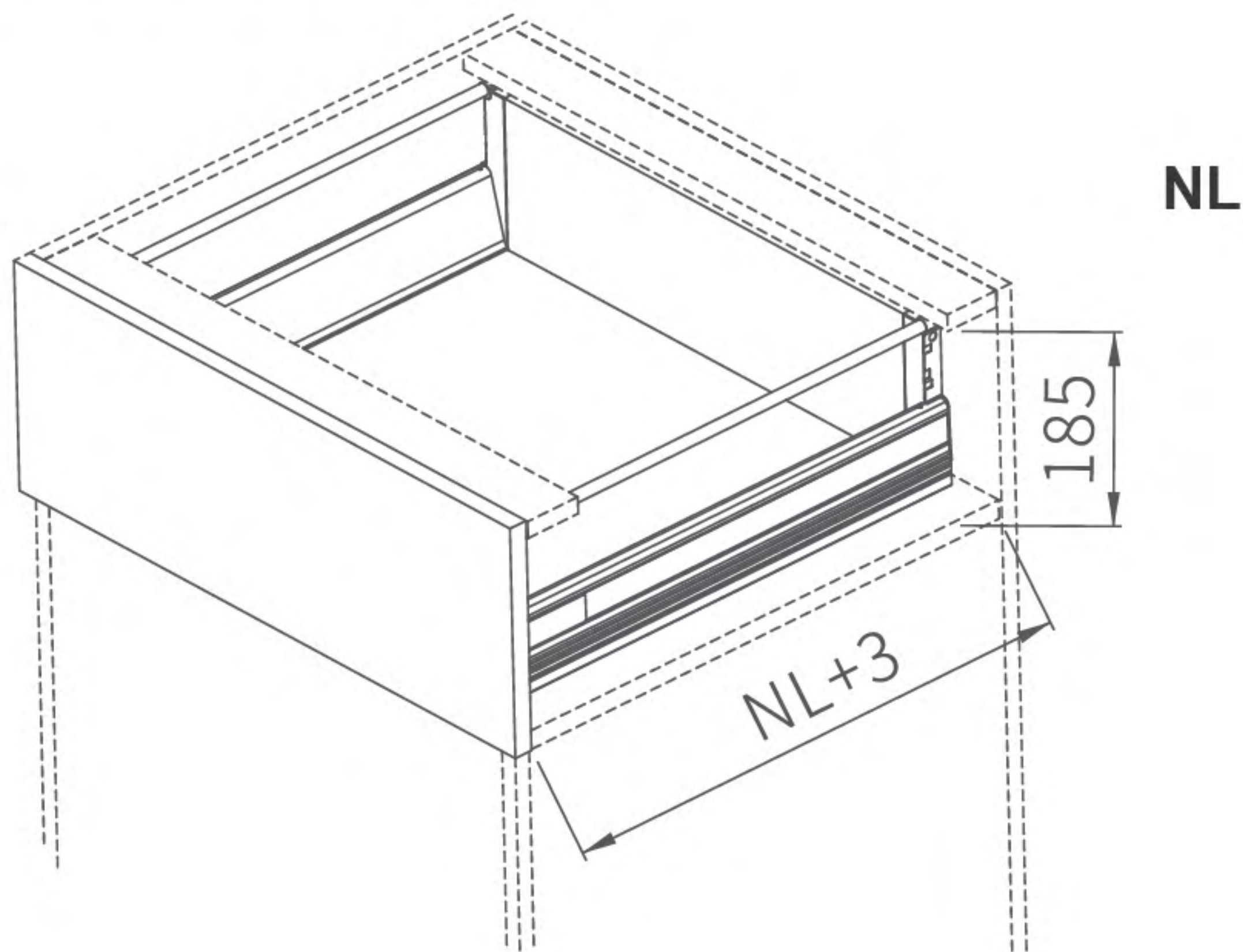
Space required
