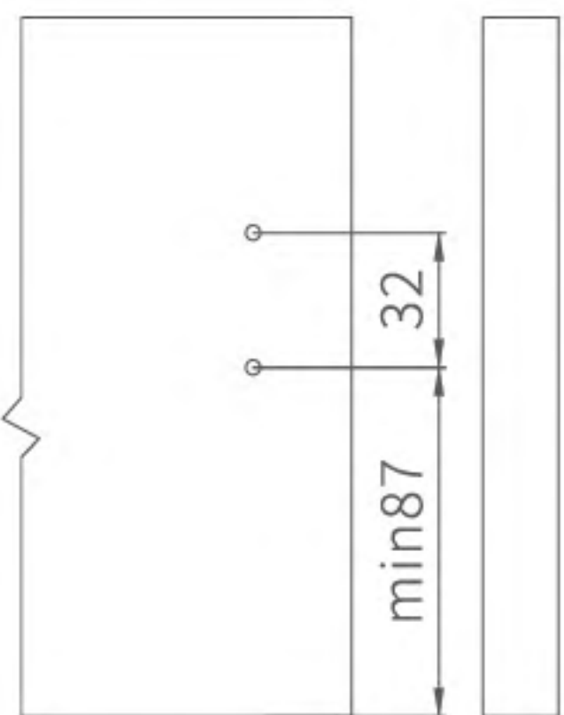
Cabinet slide mounting size
