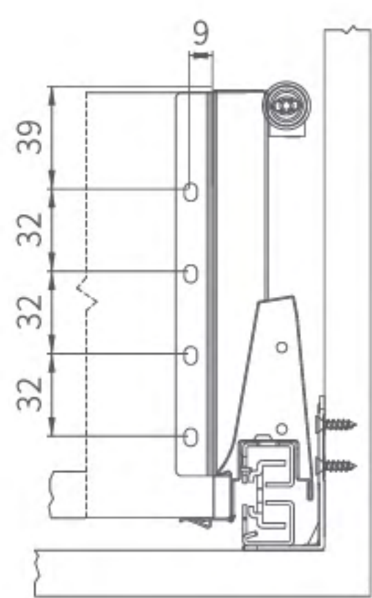
Back-panel mounting size
