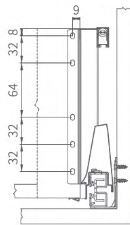
Back-panel mounting size
