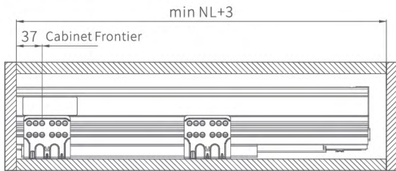
Slide mounting size
