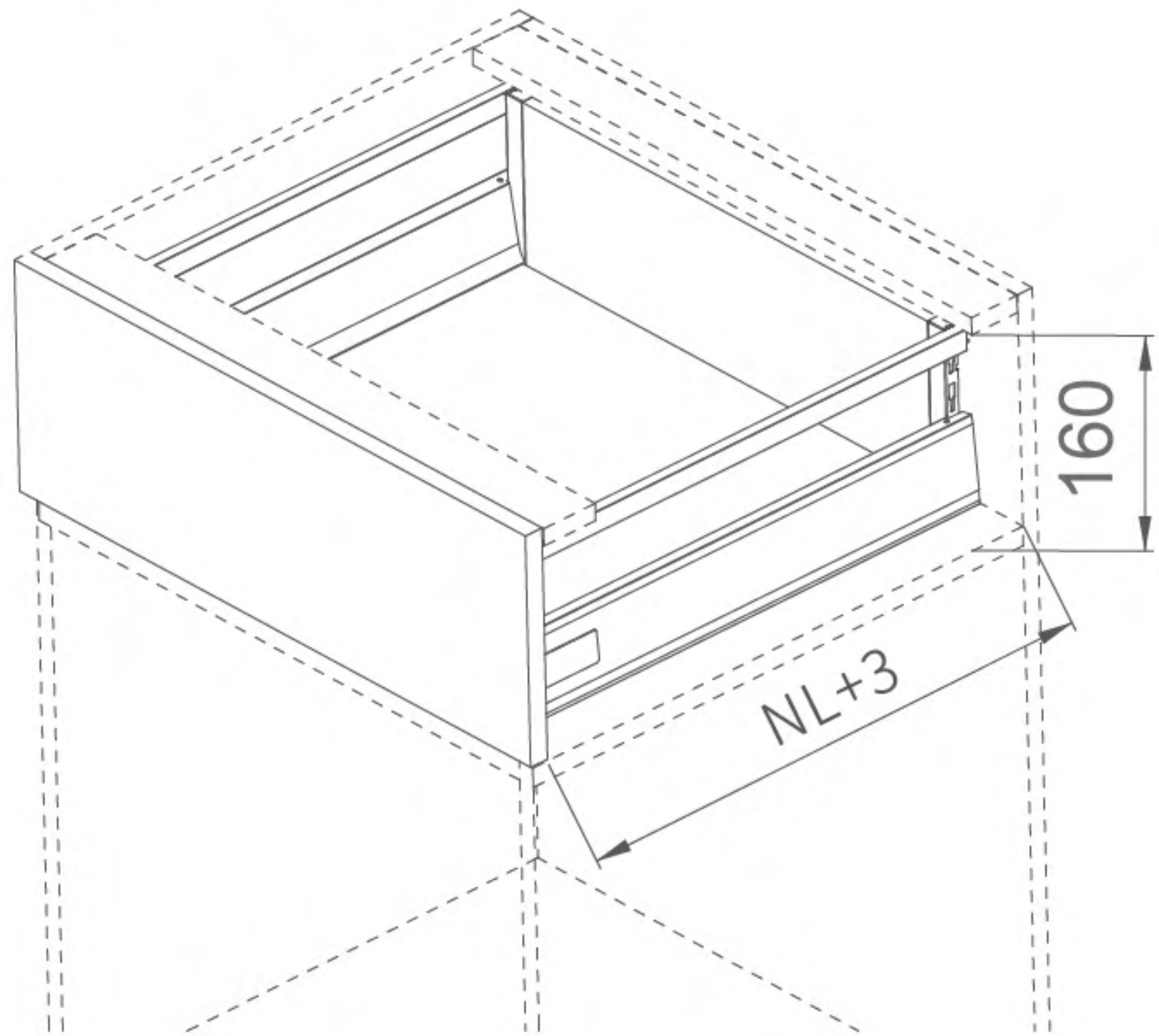
Space required
