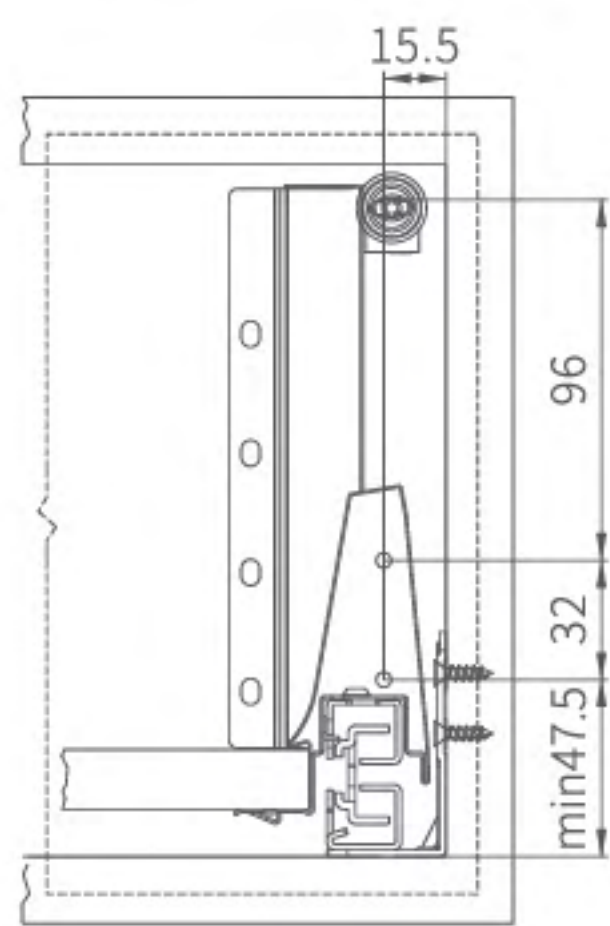
Front Connector panel mounting size
