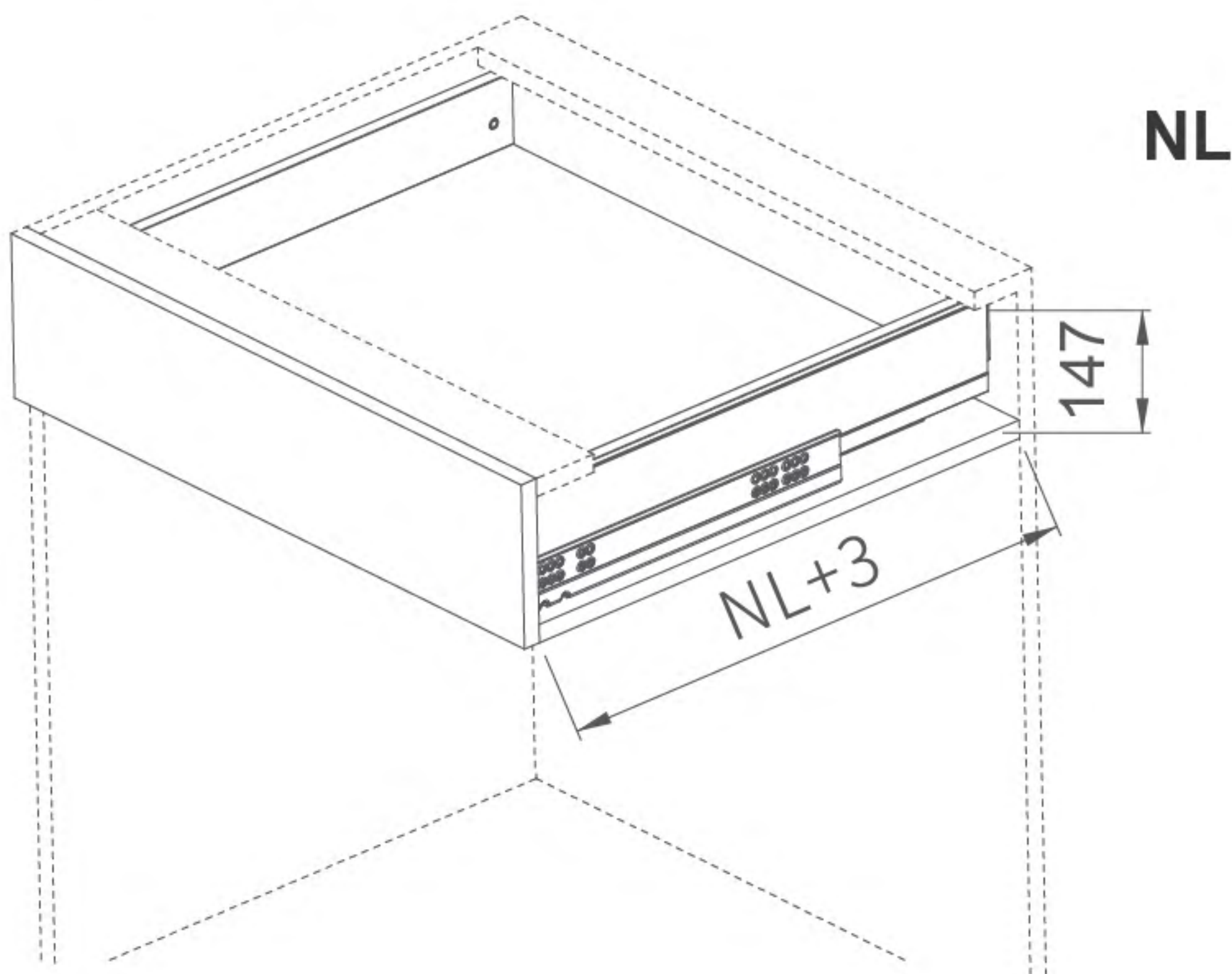
Space required
