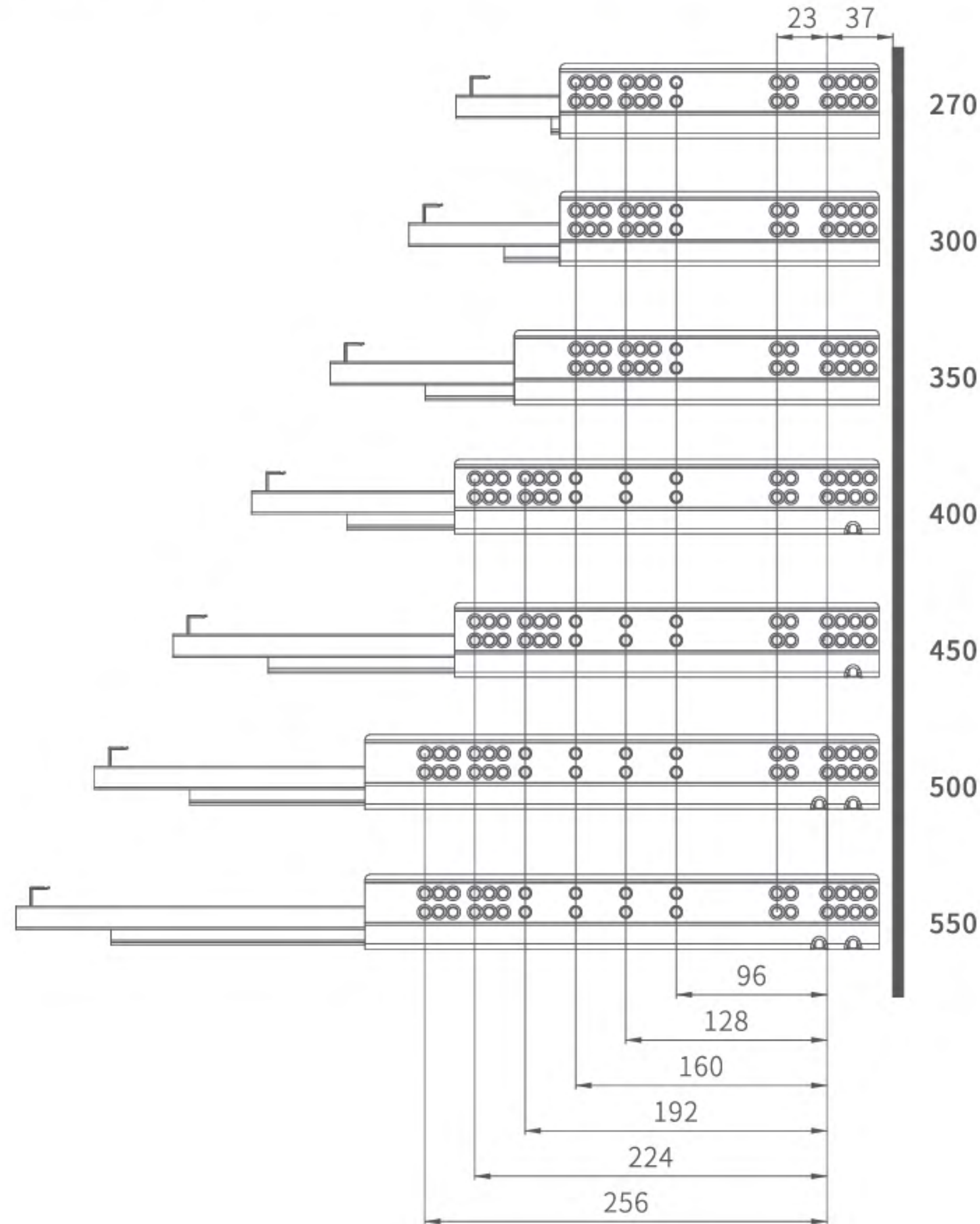
Cabinet slide mounting size
