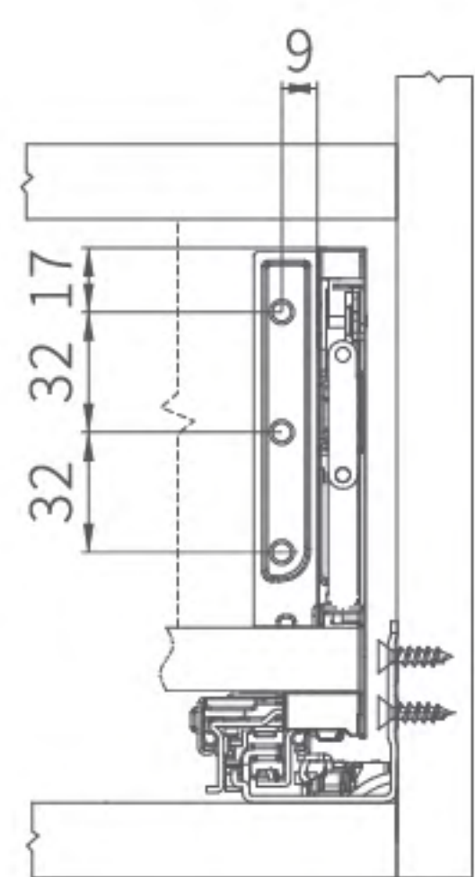
Back-panel mounting size
