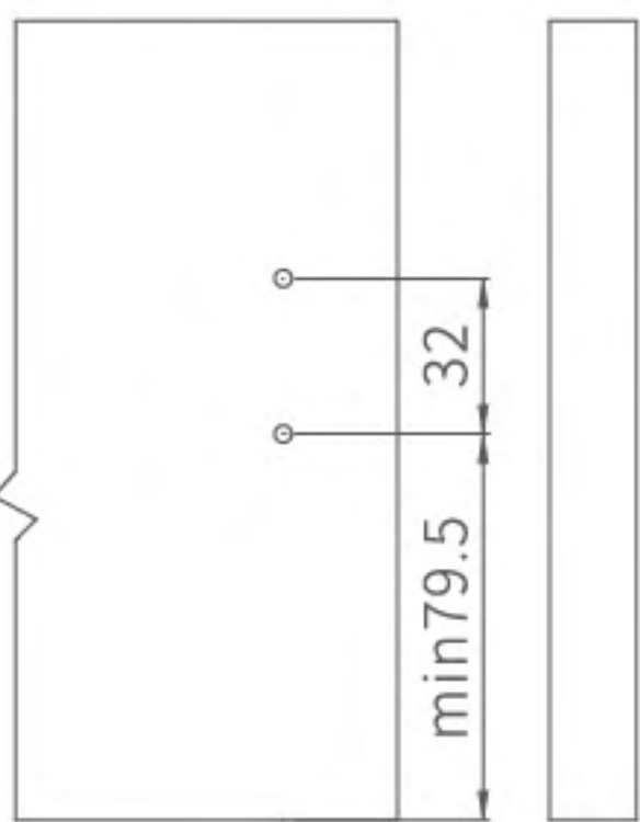
Cabinet slide mounting size
