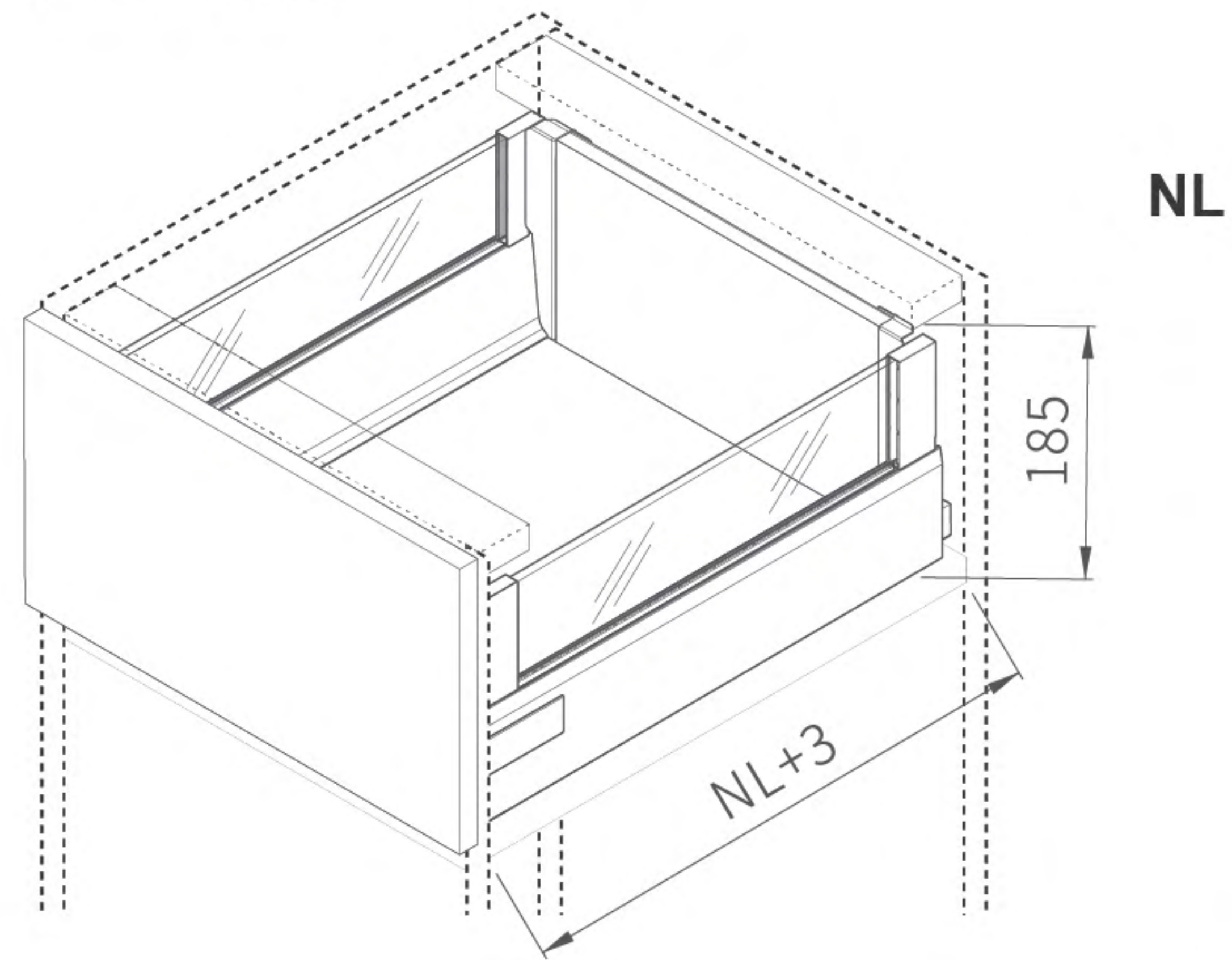
Space required
