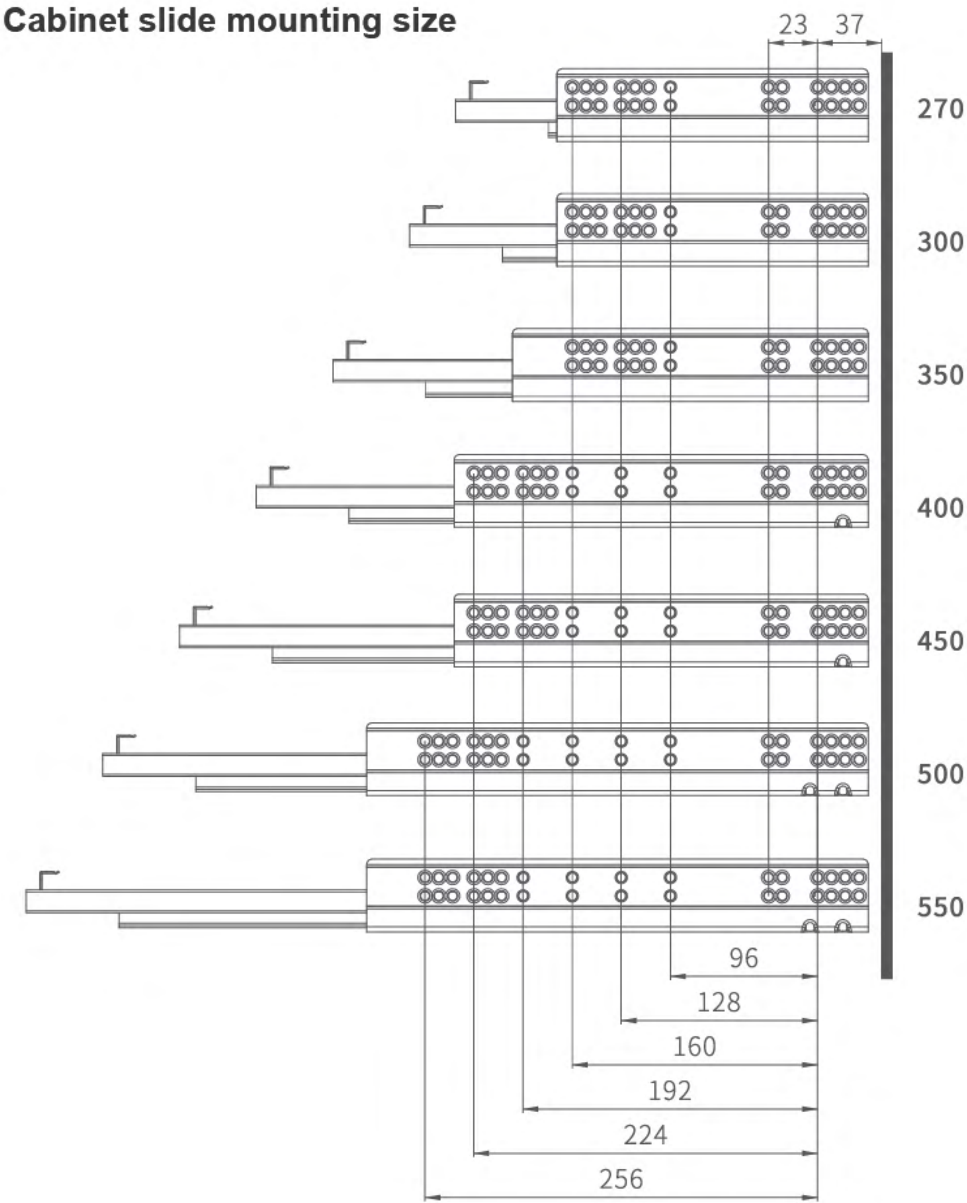
Cabinet slide mounting size
