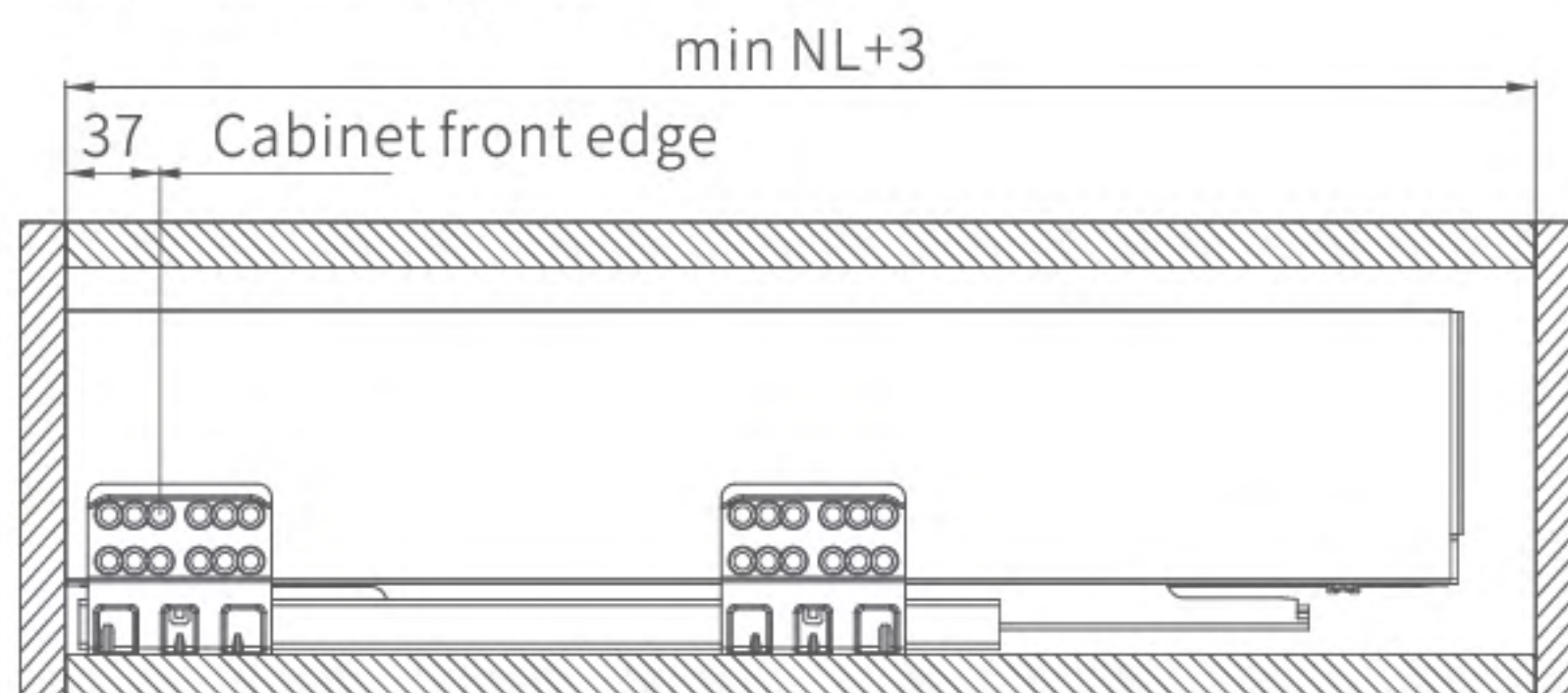
Slide mounting size
