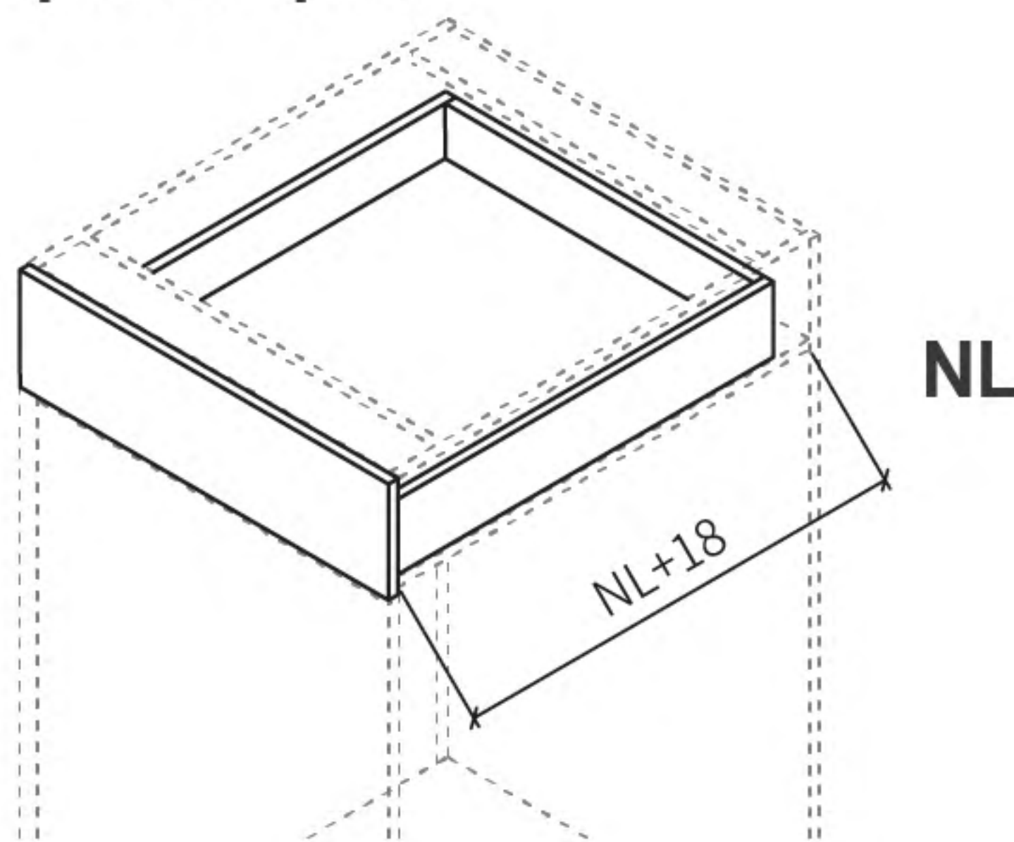
Space required
