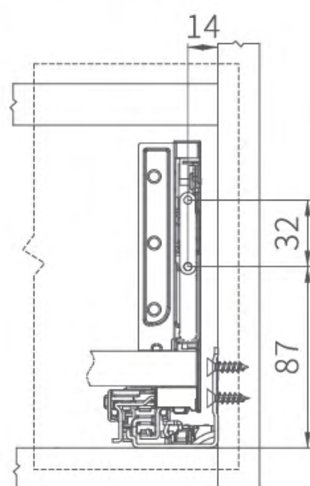
Front Connector panel mounting size
