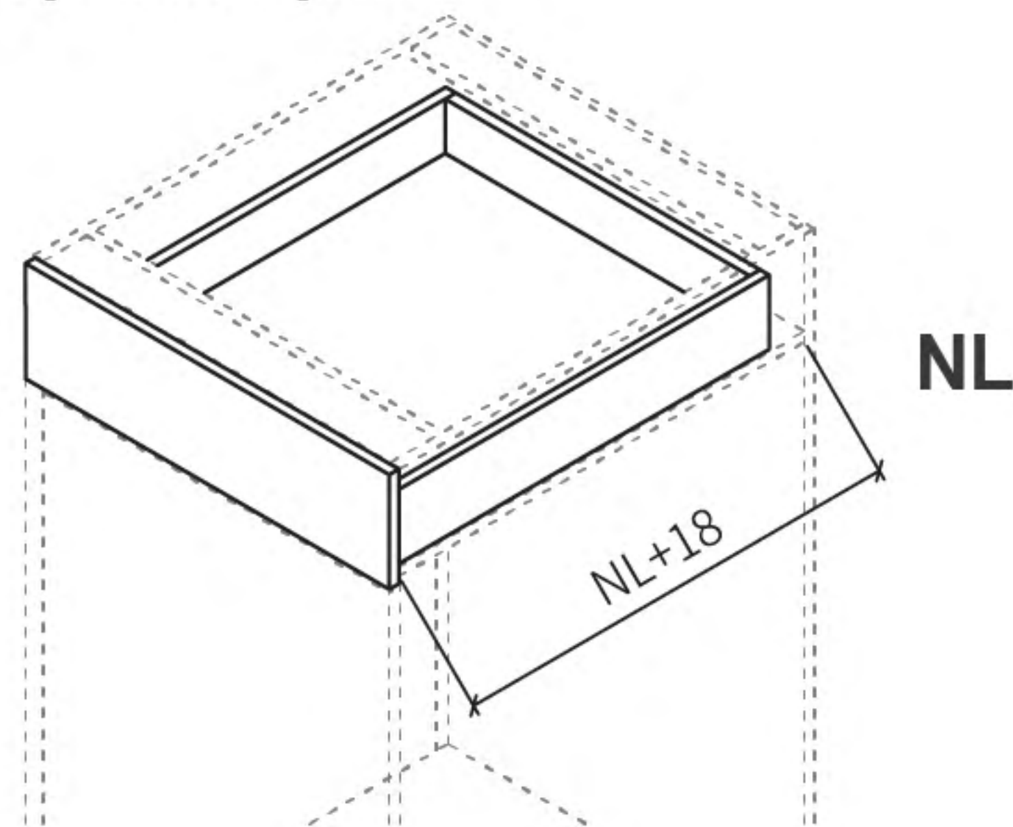
Space required
