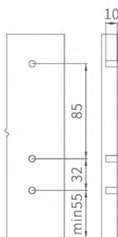
Panel hole size
