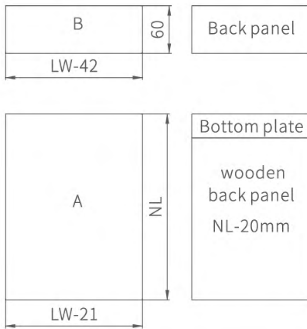
Slide mounting size
