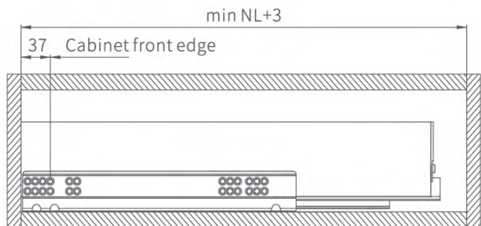
External drawer
