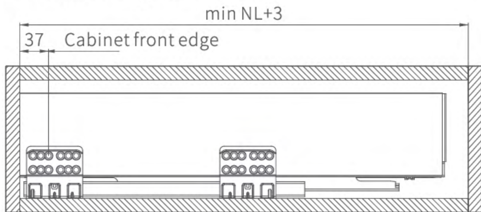
External drawer
