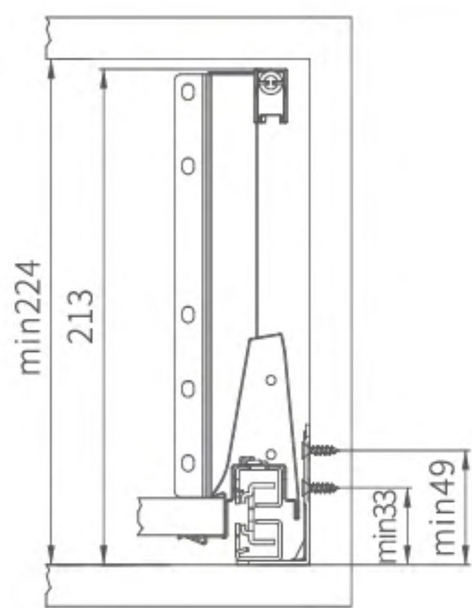
Space requirements of the inner cabinet installation
