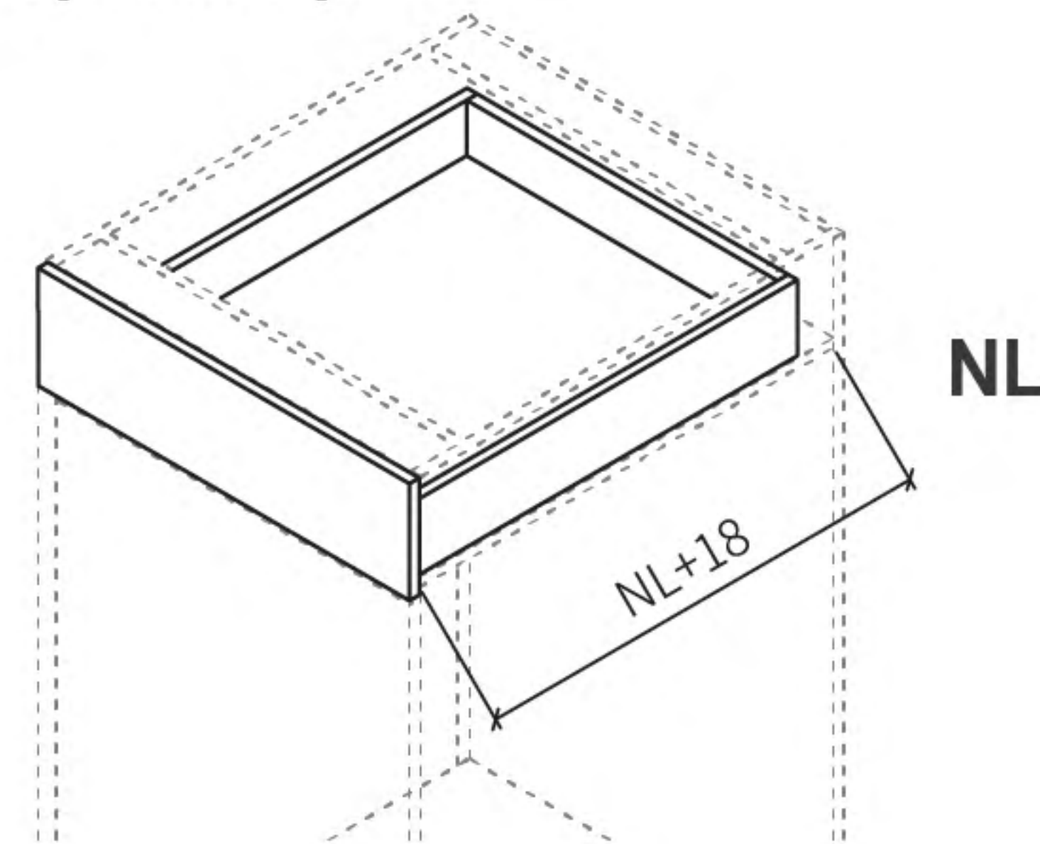
Space required
