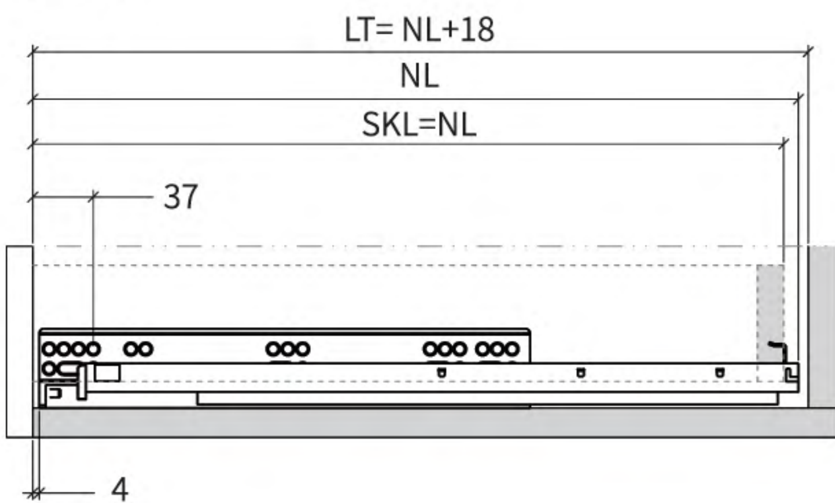
DRAWER DRILL SIZE
