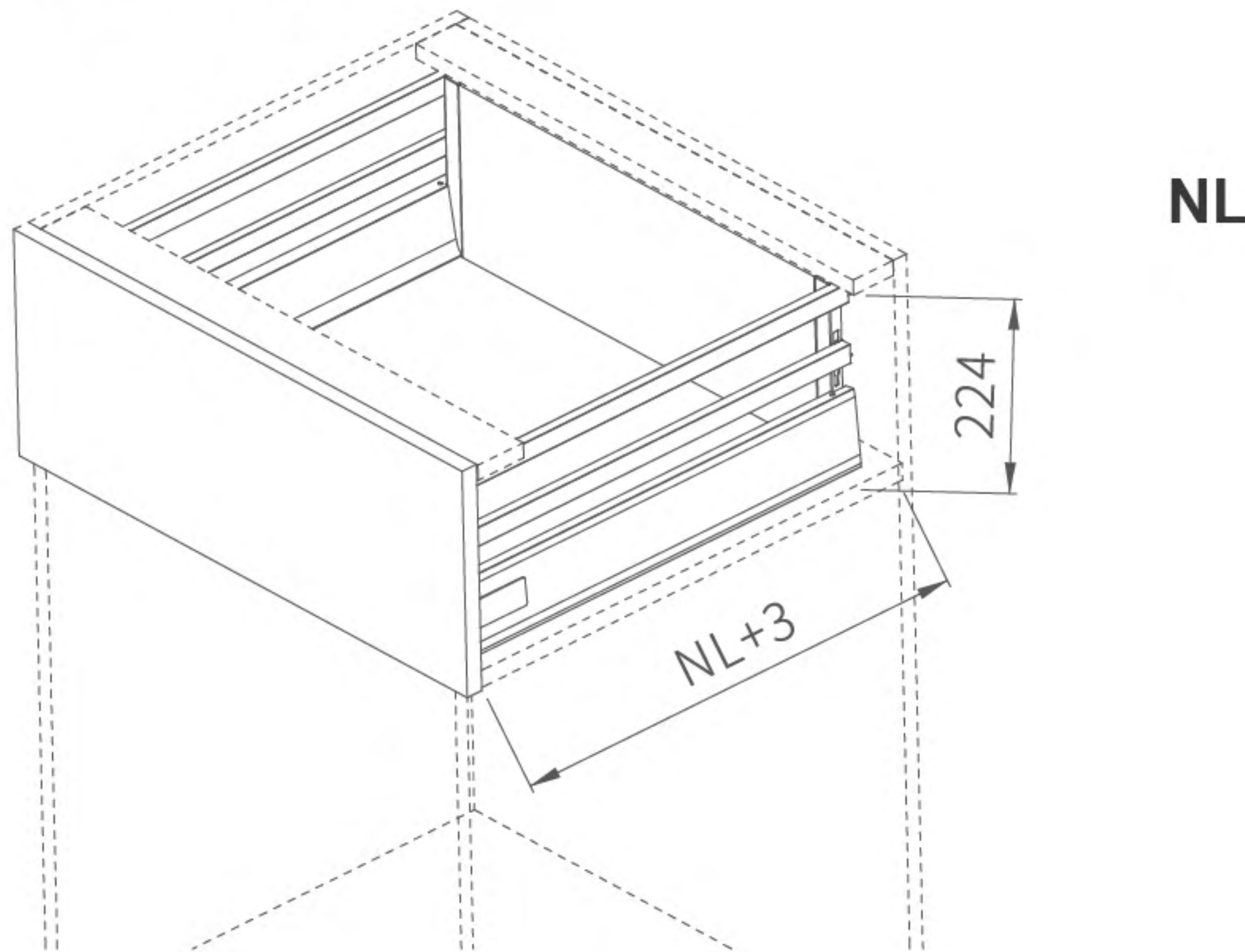
Space required
