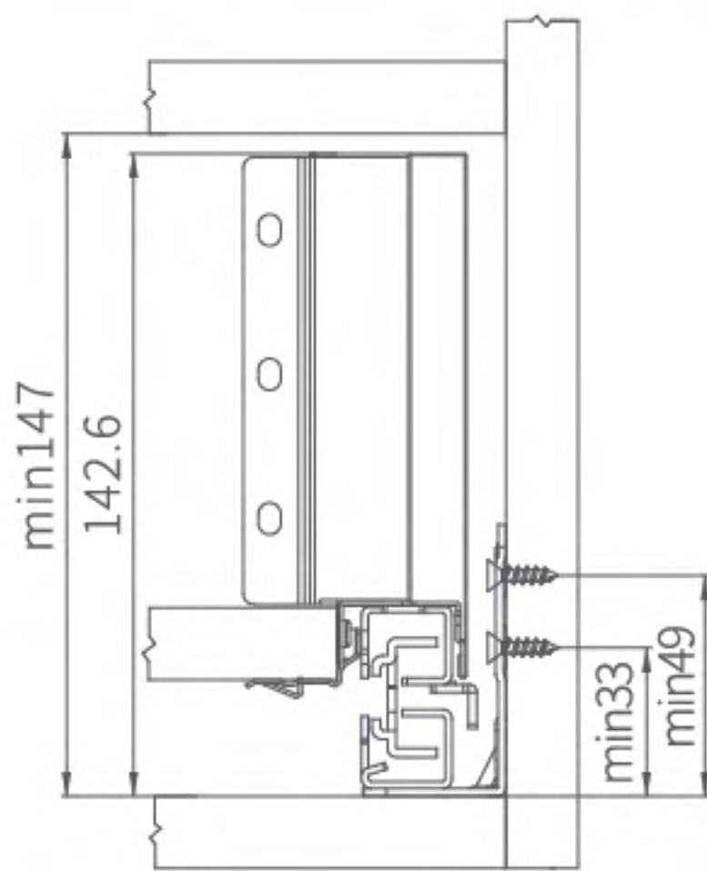
Space requirements of the inner cabinet installation
