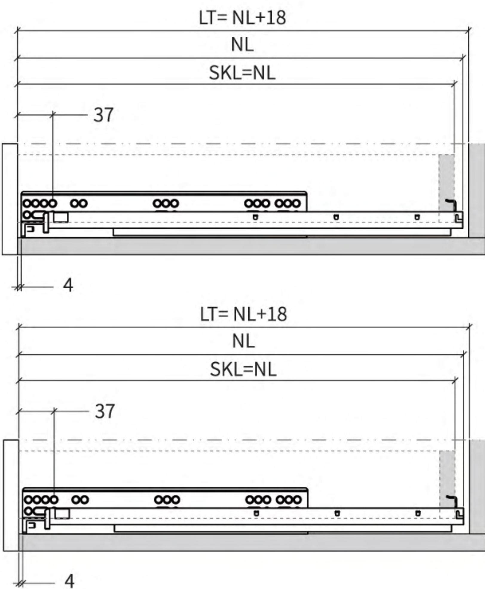
DRAWER DRILL SIZE
