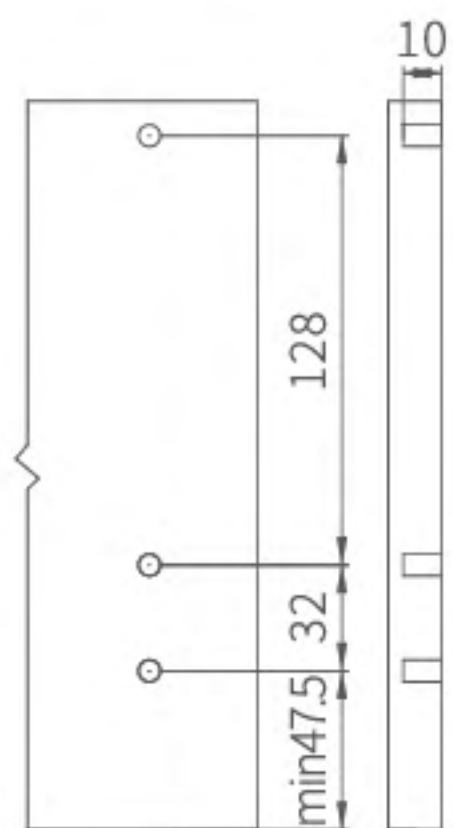
Panel hole size
