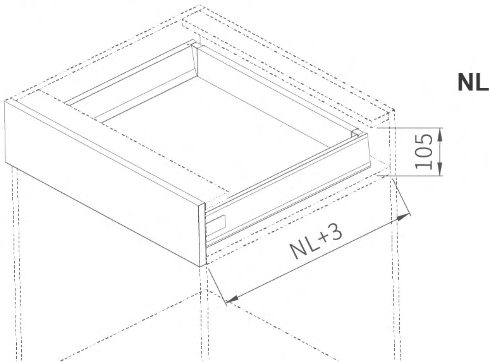
Space required
