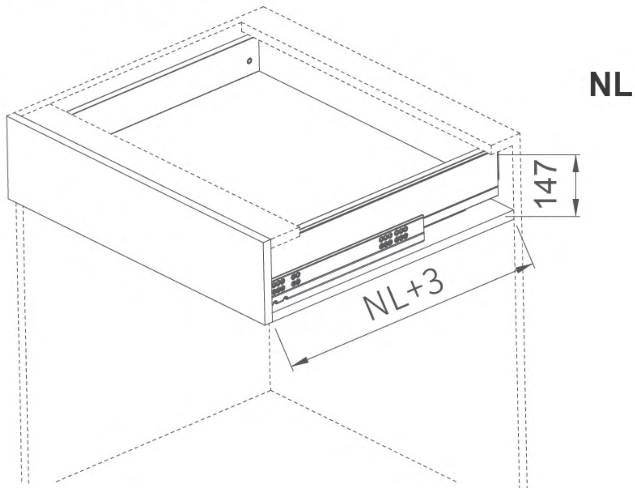
Space required
