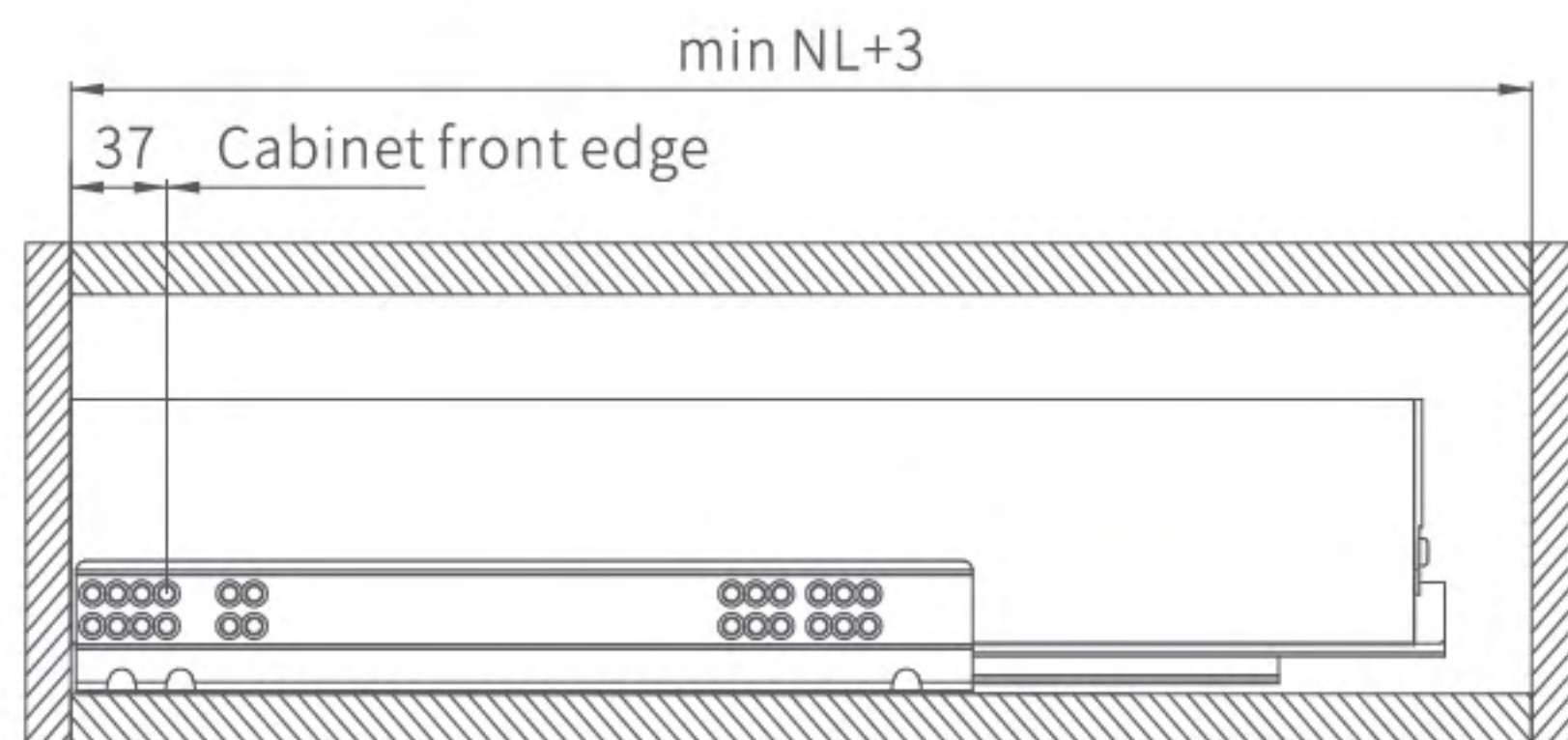
Slide mounting size
