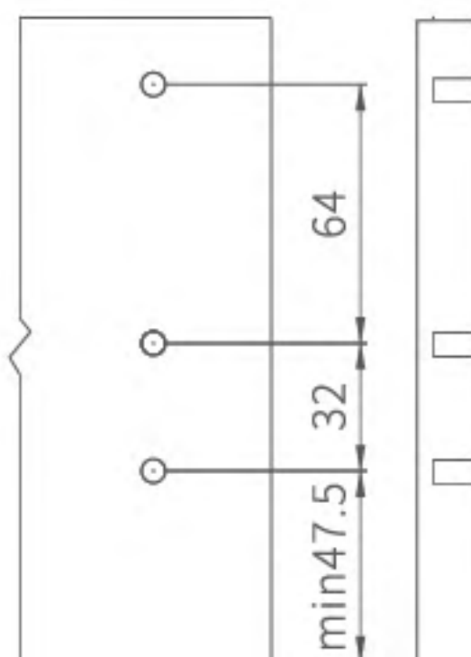
Panel hole size
