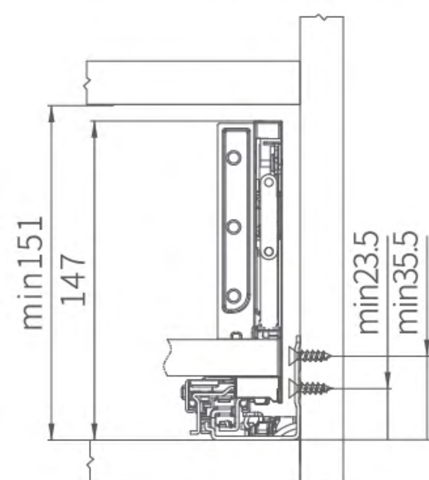
16mm(thickness)MDFcutting size
