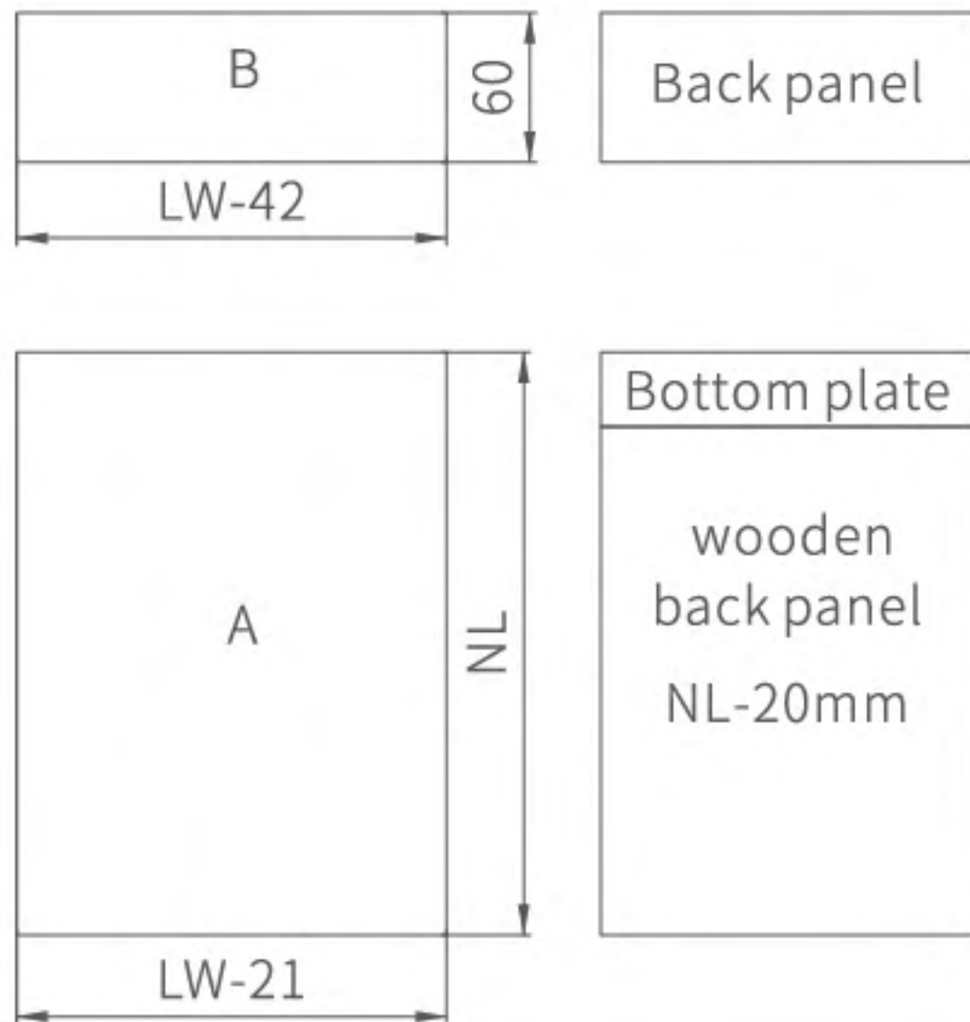
Slide mounting size
