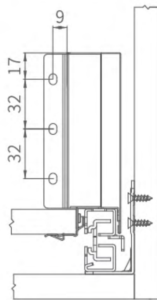
Back-panel mounting size
