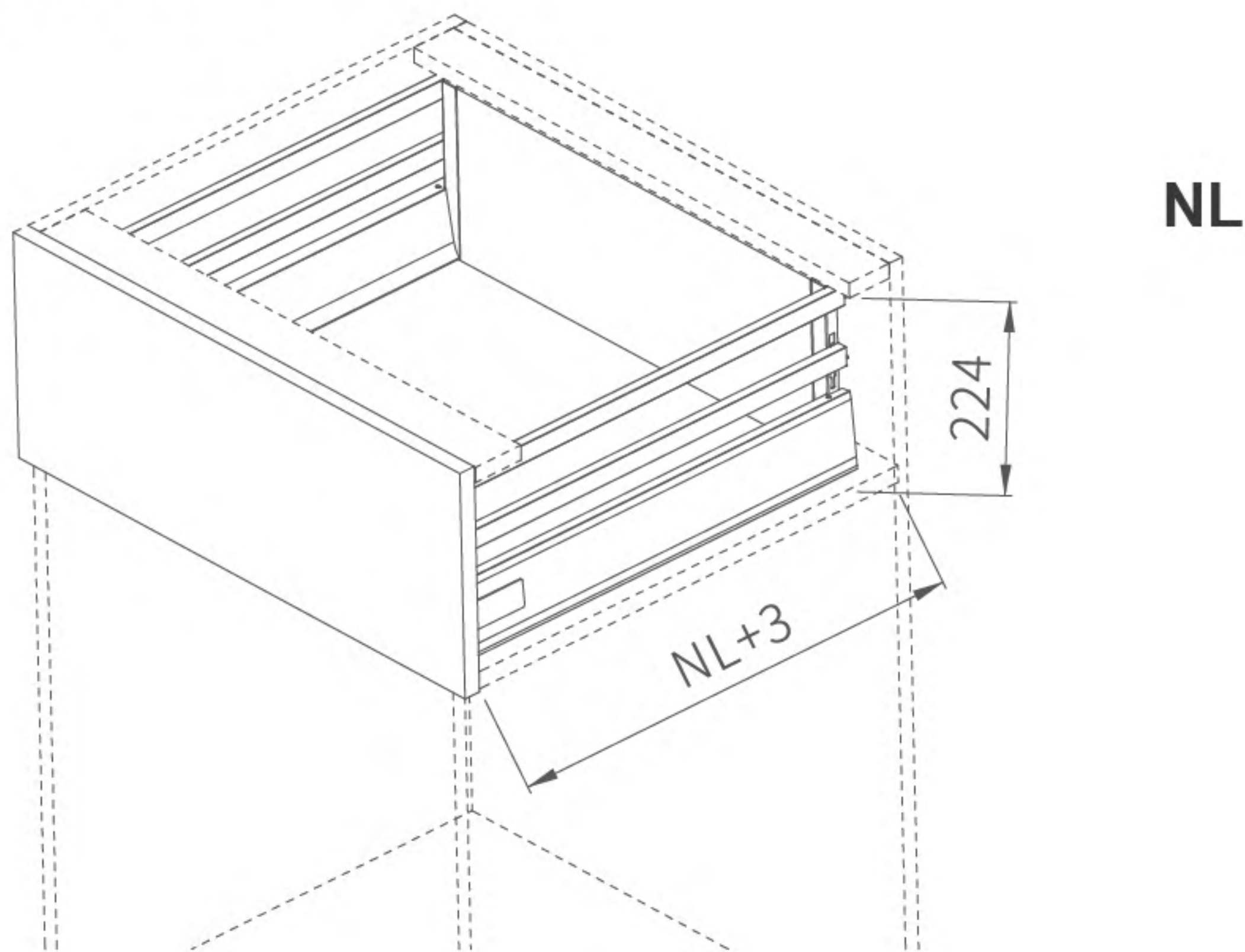
Space required
