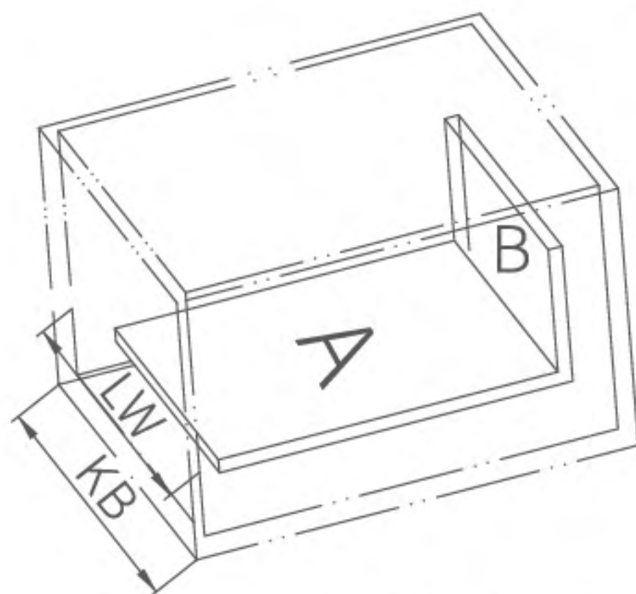
Cabinet slide mounting size
