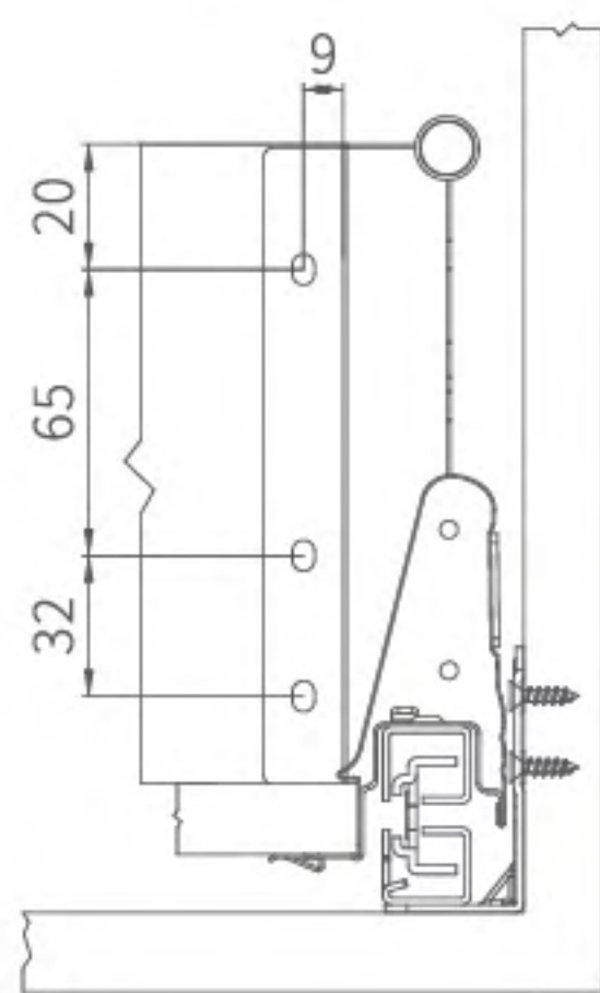
Back-panel mounting size
