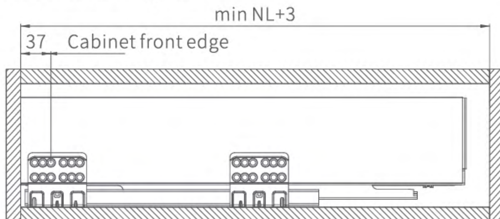
External drawer
