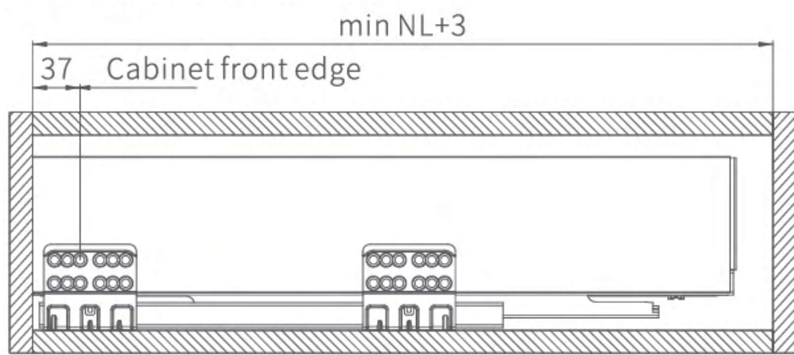
External drawer
