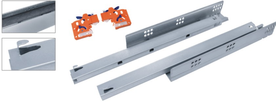
侧轨安装孔位置 Side rail mounting hole location
