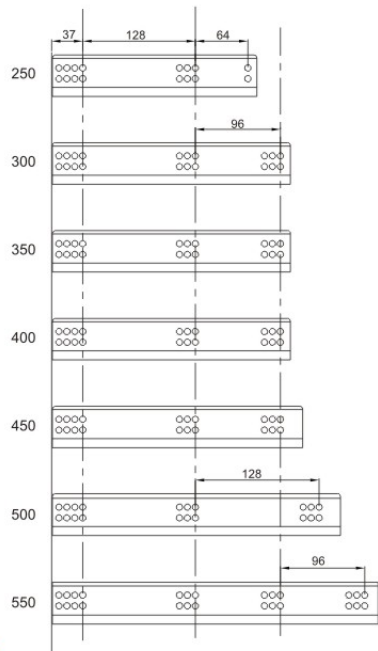
侧轨安装孔位置Side rail mounting hole location
