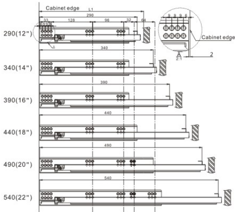
the undermount slide installation hole system
