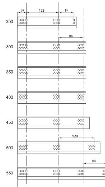
侧轨安装孔位置Side rail mounting hole location
