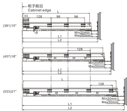
侧轨安装孔位置Side rail mounting hole location
