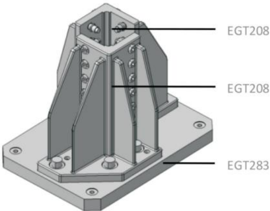
尺寸: 315mm x 225mm x 248mm
