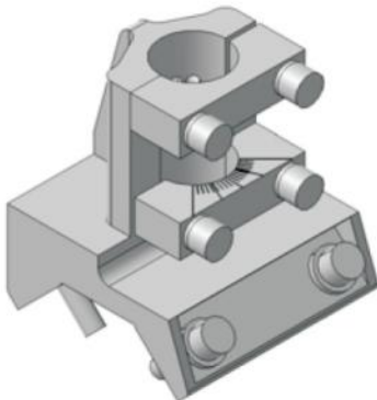
尺寸: 99mm x 81mm x 88mm
