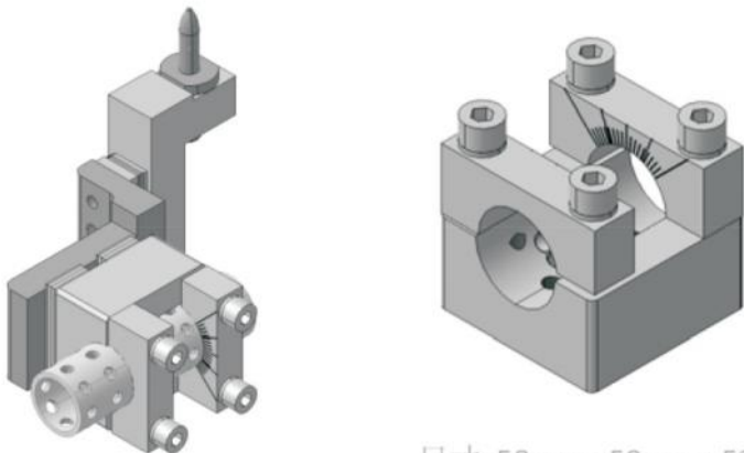
尺寸: 58mm x 58mm x 53mm
