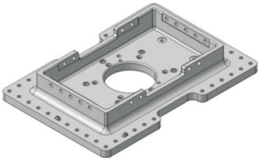
尺寸: 330mm x 480mm x 74mm
