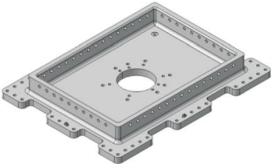
尺寸: 630mm x 480mm x 79mm
