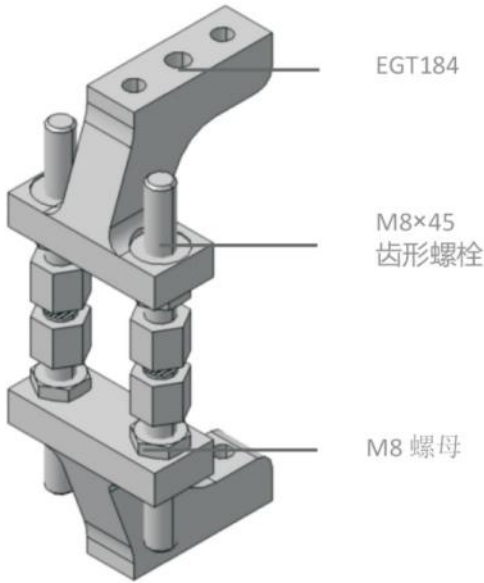
尺寸: 138mm x 50mm x 57mm
