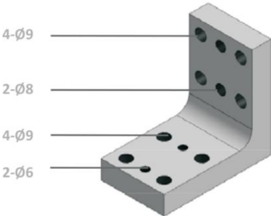
尺寸: 50mm x 80mm x 85mm
