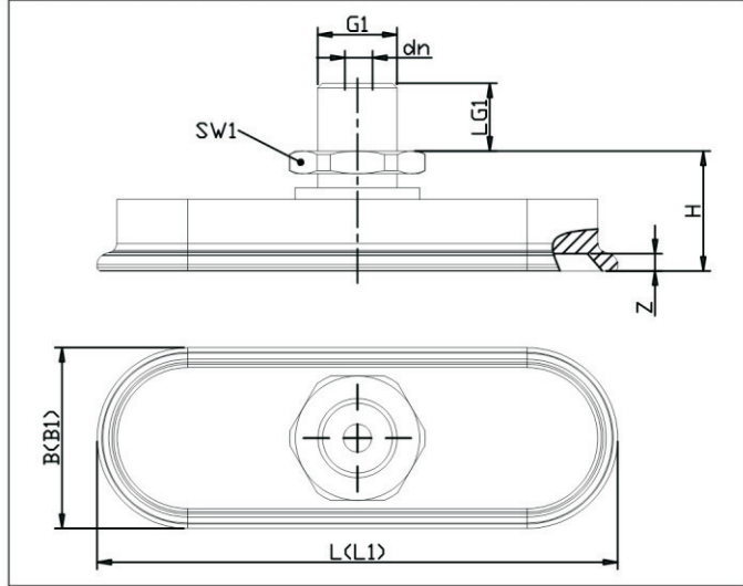
MAOF 50 × 16 至 120 × 60 AG
