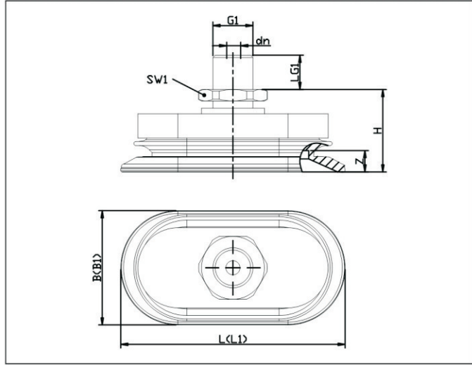
MAOB 60 × 30 至 110 × 55 AG
