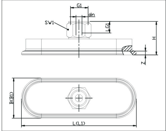
MAOF 50 × 16 至 120 × 60 IG
