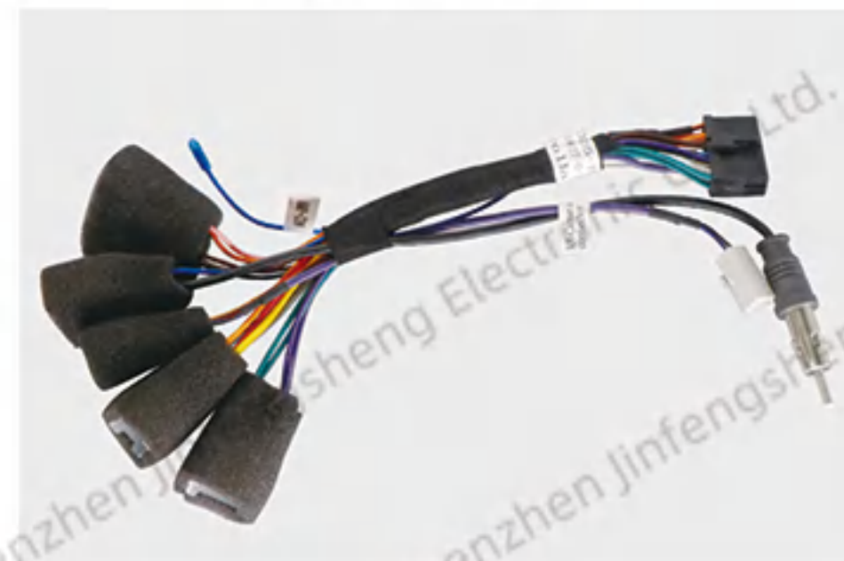
Automotive 20-Pole Low-Current Power Wiring Harness
