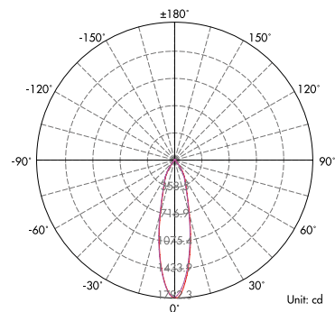
Light Distribution Curve (3000K, 1x38°) .....
