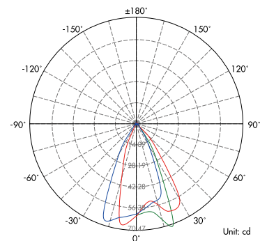
Light Distribution Curve (3000K, 25°) .....
