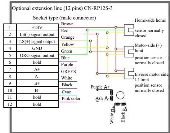
YK-L6030U-SSR-2-615 Wiring Diagram
