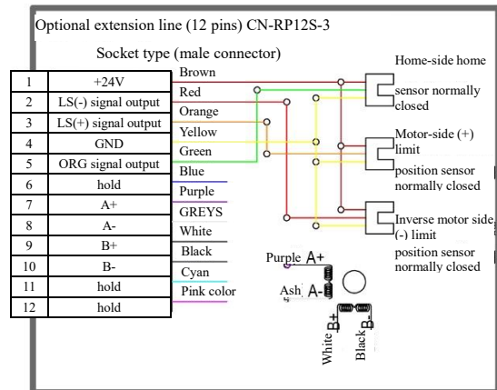
YK-L6030U-SSL-2-615 Wiring Diagram
