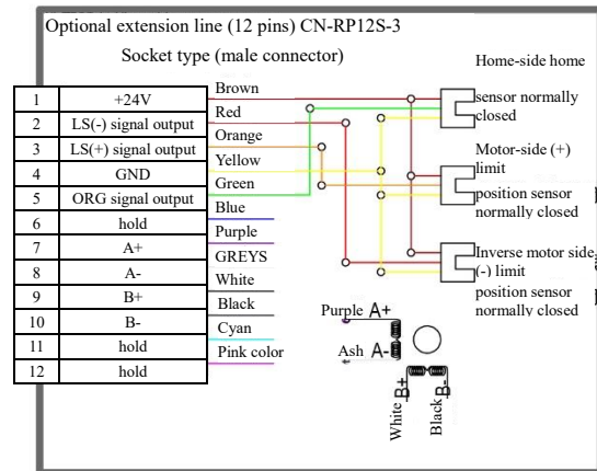
YK-L6020U-SSR-2C-615 Wiring Diagram
