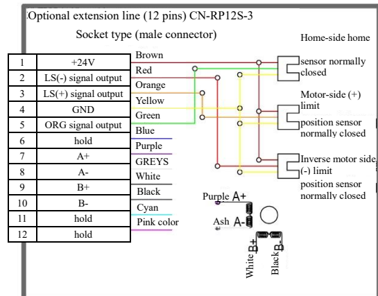
Connection diagram
