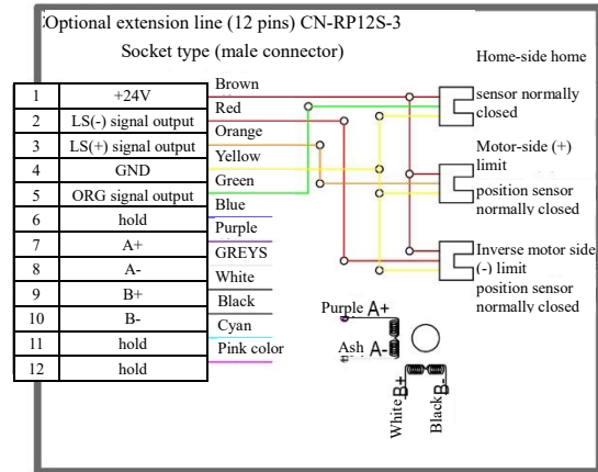
YK-L6020U-SSL-2C-615 Wiring Diagram
