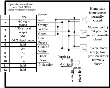
YK-C6050U-ASL-2C-615 Wiring Diagram
