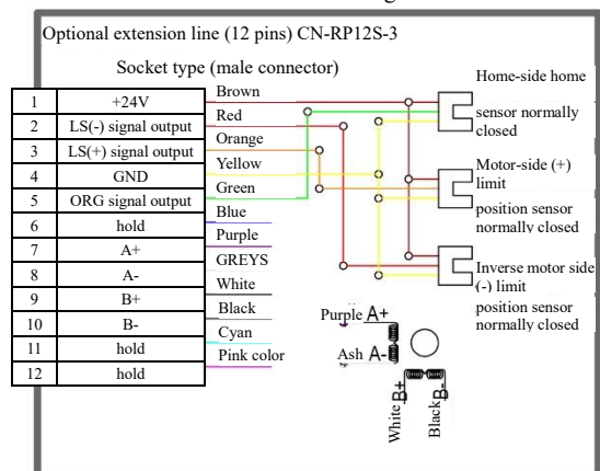
Connection diagram
