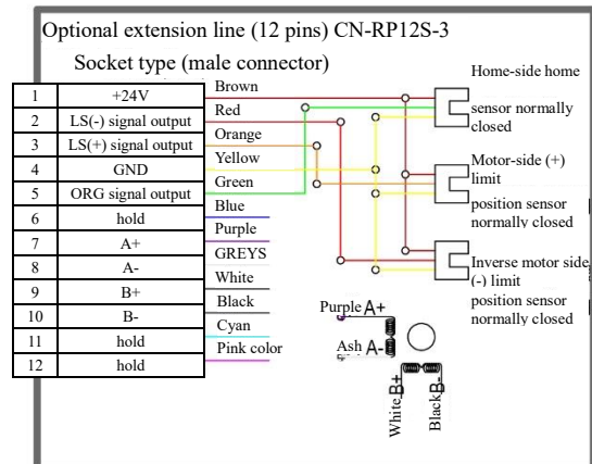
YK-HL8050U-SSN-2C-815 Wiring Diagram
