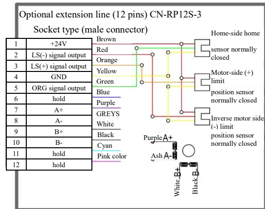
YK-HL8050U-SSN-2-815 Wiring Diagram
