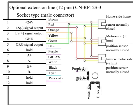
YK-HL8020U-SSN-2C-815 Wiring Diagram
