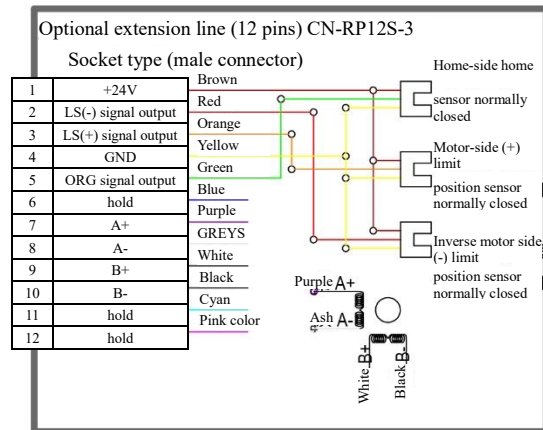
YK-HL8020U-SSN-2-815 Wiring Diagram
