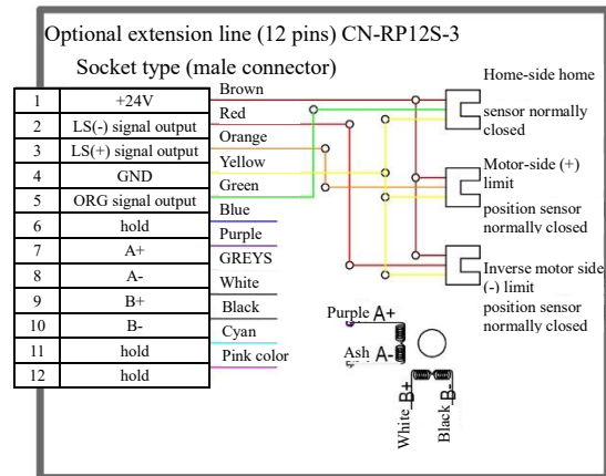
YK-HL6050U-SSN-2-815 Wiring Diagram
