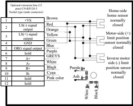
YK-C6075U-ASR-2C-615 Wiring Diagram
