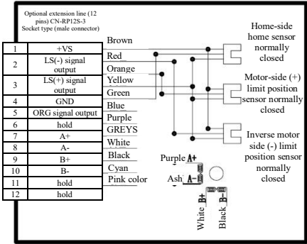
YK-C6075U-ASL-2C-615 Wiring Diagram
