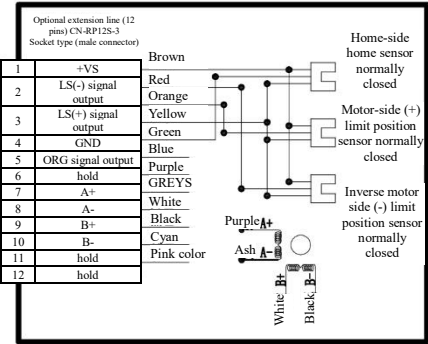
YK-C60125U-ASR-2-615 Wiring Diagram
