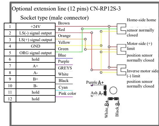
YK-C60125U-ASL-2C-615 Wiring Diagram
