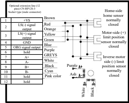
YK-C60100U-ASL-2-615 Wiring Diagram
