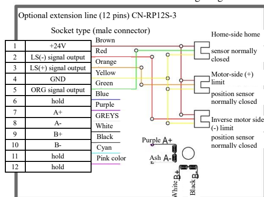
YK-L4015U-SSL-2C-615 Wiring Diagram
