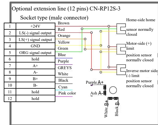
YK-L4015U-SSL-2-615 Wiring Diagram
