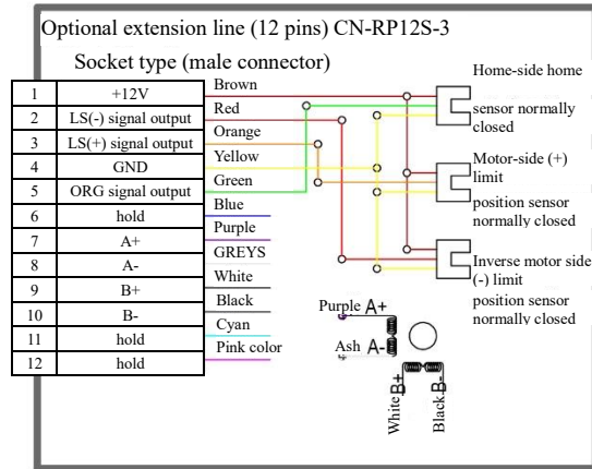
YK-HL8030U-SSN-2C-815 Wiring Diagram
