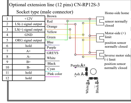
YK-R8016U-ASN-2C-615 Wiring Diagram
