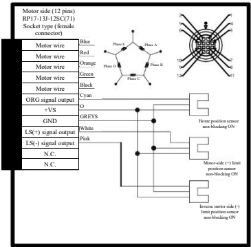
YK-HL6030G-SGN-5-815 Wiring Diagram
