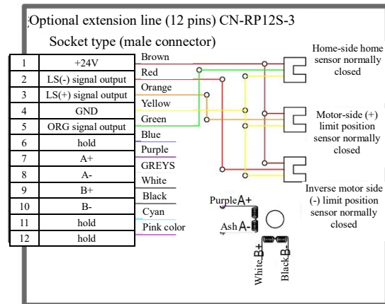
YK-HL6020U-SSN-2-815 Wiring Diagram
