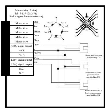
YK-HL6020G-SGN-5-815 Wiring Diagram
