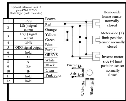
YK-C60100U-ASL-2C-615 Wiring Diagram
