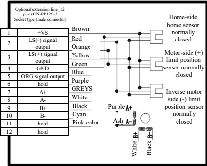
YK-C60100U-ASL-2-615 Wiring Diagram
