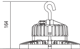
JD-HB032A-100W
