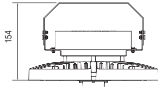
JD-HB032B-W-150W
