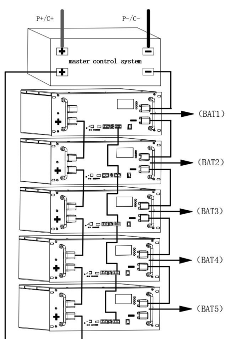
Part1:100A max, the Wiring diagram for the parallel connection of 5 pcs
