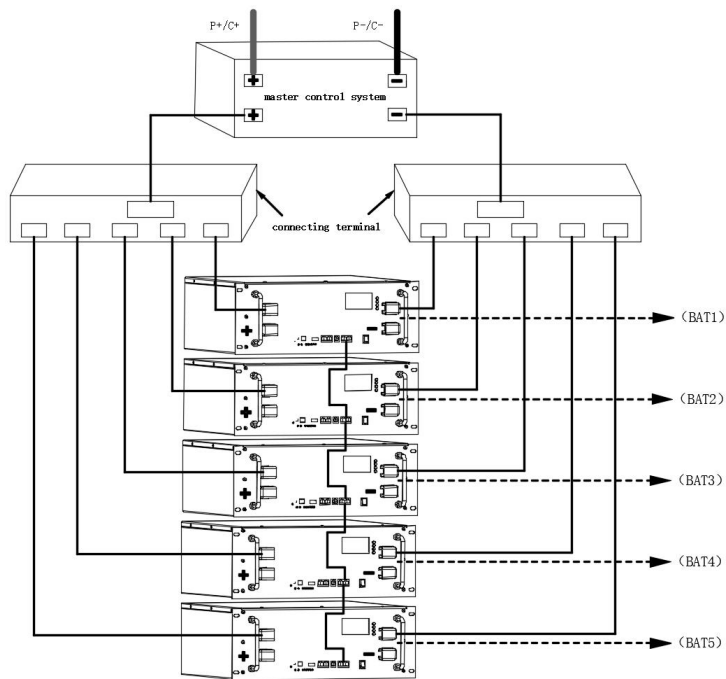
Part2:200A max, the Wiring diagram for the parallel connection of 5 pcs
