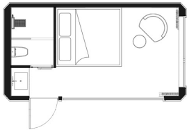
* 产品平面布局图 (仅供参考) *Product floor plan layout (for reference only)
