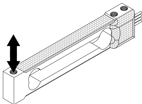
Load direction
