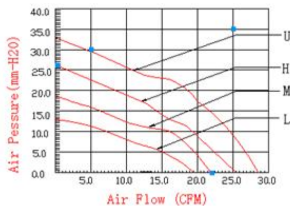
Characteristic Curve
