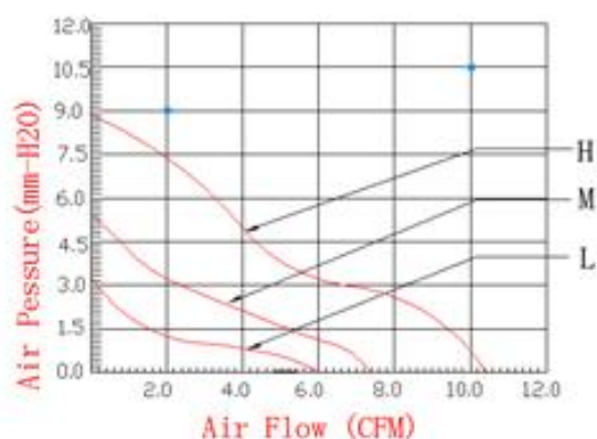
Characteristic Curve
