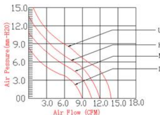
Characteristic Curve
