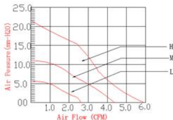
Characteristic Curve
