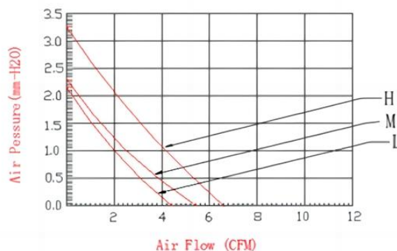
Characteristic Curve
