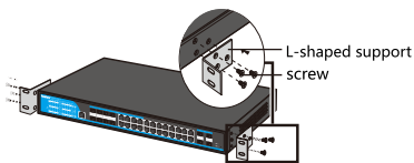
Figure 1.1.1 installation diagram of switch
