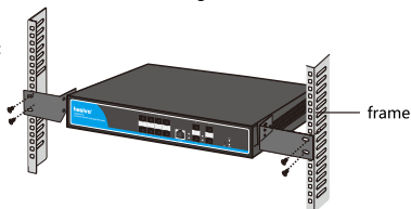
Figure 1.1.2 installation diagram of switch
