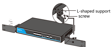
Figure 1.1.1 installation diagram of switch
